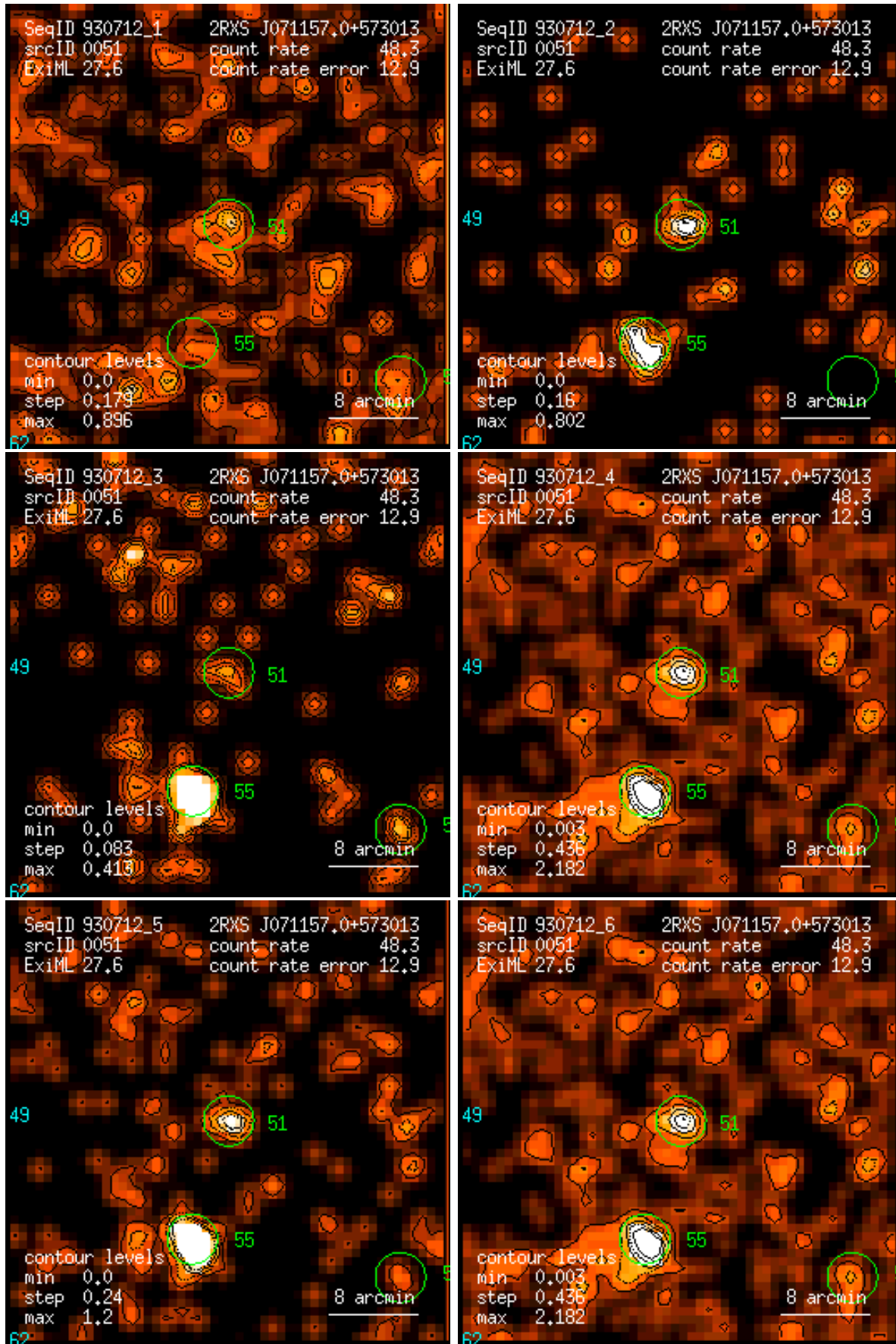
Figure 51: RASS 930712: detection 0051: band rate images, Gaussian filter: (1) PSPC channels 11 – 41, (2) 52 – 90, (3) 91 – 201, (4) 11 – 235, (5) 52 – 201, (6) 11 – 201. Broad band rates in counts/ks. Band rate contour levels in counts/ks/arcmin 2 .
