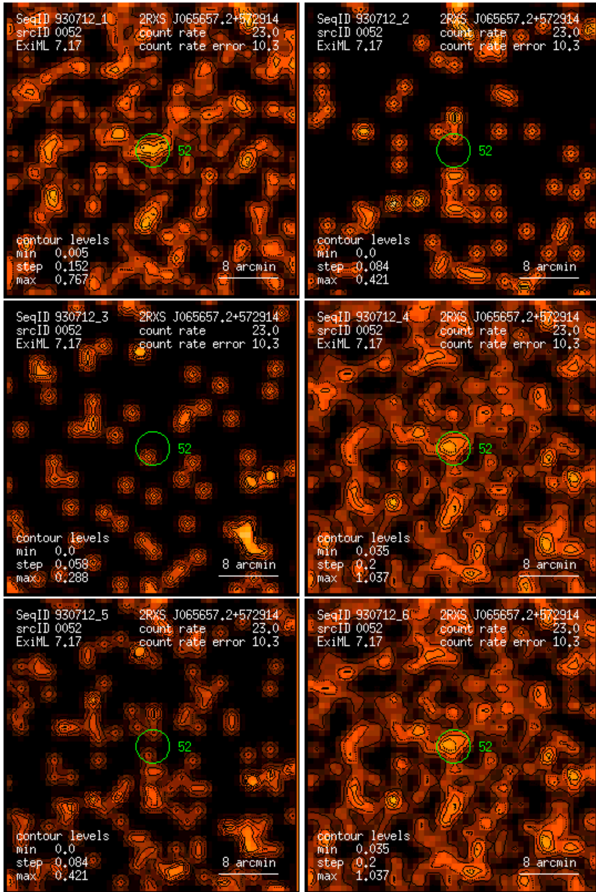
Figure 52: RASS 930712: detection 0052: band rate images, Gaussian filter: (1) PSPC channels 11 – 41, (2) 52 – 90, (3) 91 – 201, (4) 11 – 235, (5) 52 – 201, (6) 11 – 201. Broad band rates in counts/ks. Band rate contour levels in counts/ks/arcmin 2 .
