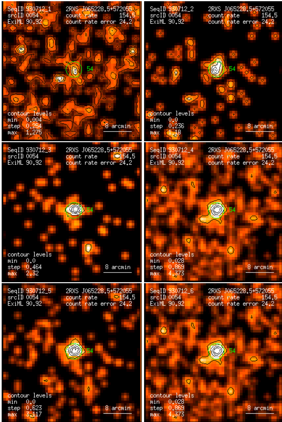
Figure 54: RASS 930712: detection 0054: band rate images, Gaussian filter: (1) PSPC channels 11 – 41, (2) 52 – 90, (3) 91 – 201, (4) 11 – 235, (5) 52 – 201, (6) 11 – 201. Broad band rates in counts/ks. Band rate contour levels in counts/ks/arcmin 2 .
