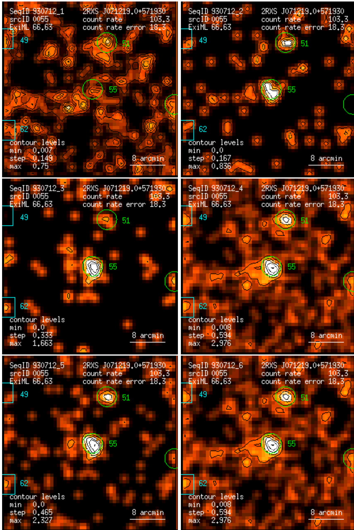
Figure 55: RASS 930712: detection 0055: band rate images, Gaussian filter: (1) PSPC channels 11 – 41, (2) 52 – 90, (3) 91 – 201, (4) 11 – 235, (5) 52 – 201, (6) 11 – 201. Broad band rates in counts/ks. Band rate contour levels in counts/ks/arcmin 2 .
