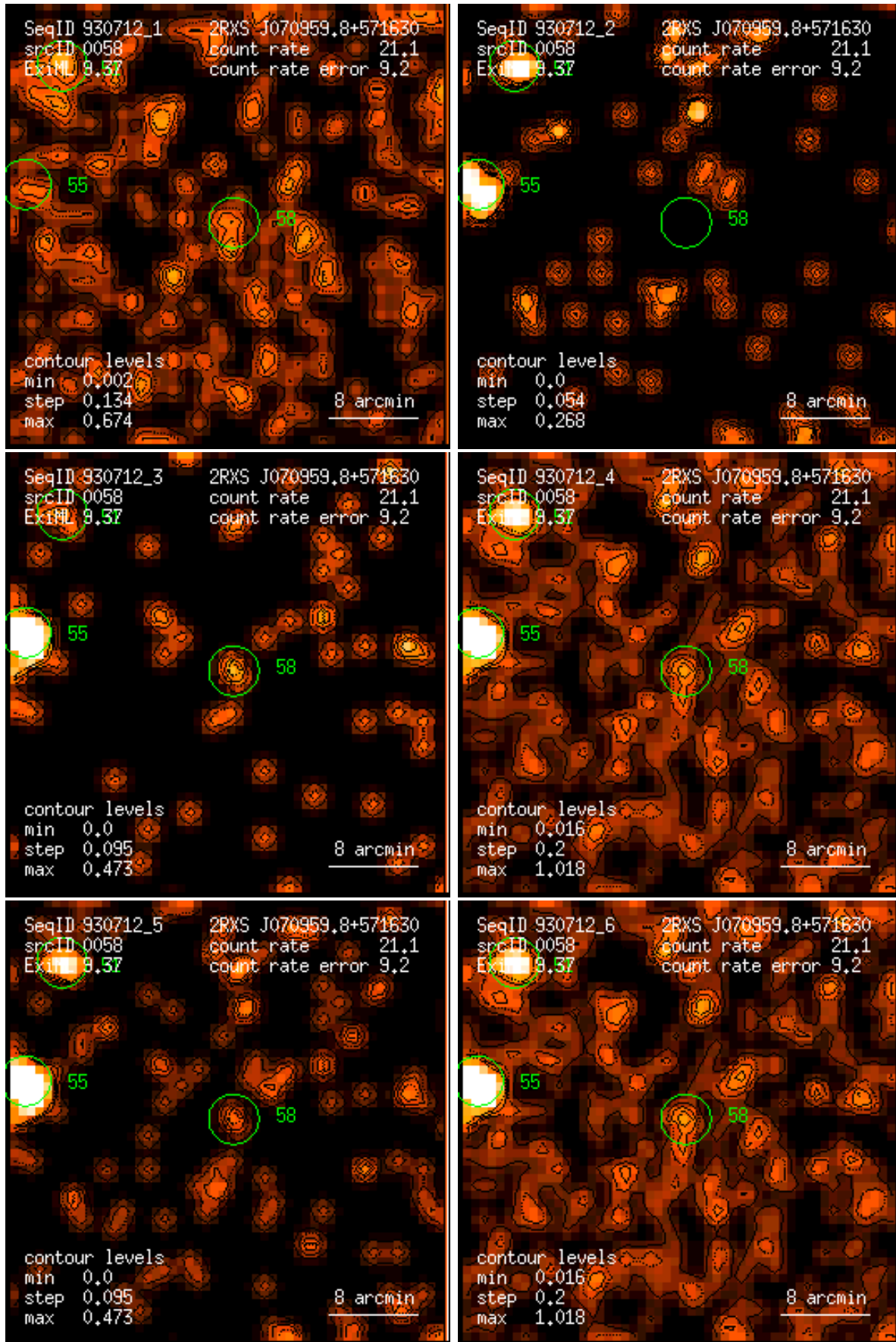
Figure 58: RASS 930712: detection 0058: band rate images, Gaussian filter: (1) PSPC channels 11 – 41, (2) 52 – 90, (3) 91 – 201, (4) 11 – 235, (5) 52 – 201, (6) 11 – 201. Broad band rates in counts/ks. Band rate contour levels in counts/ks/arcmin 2 .
