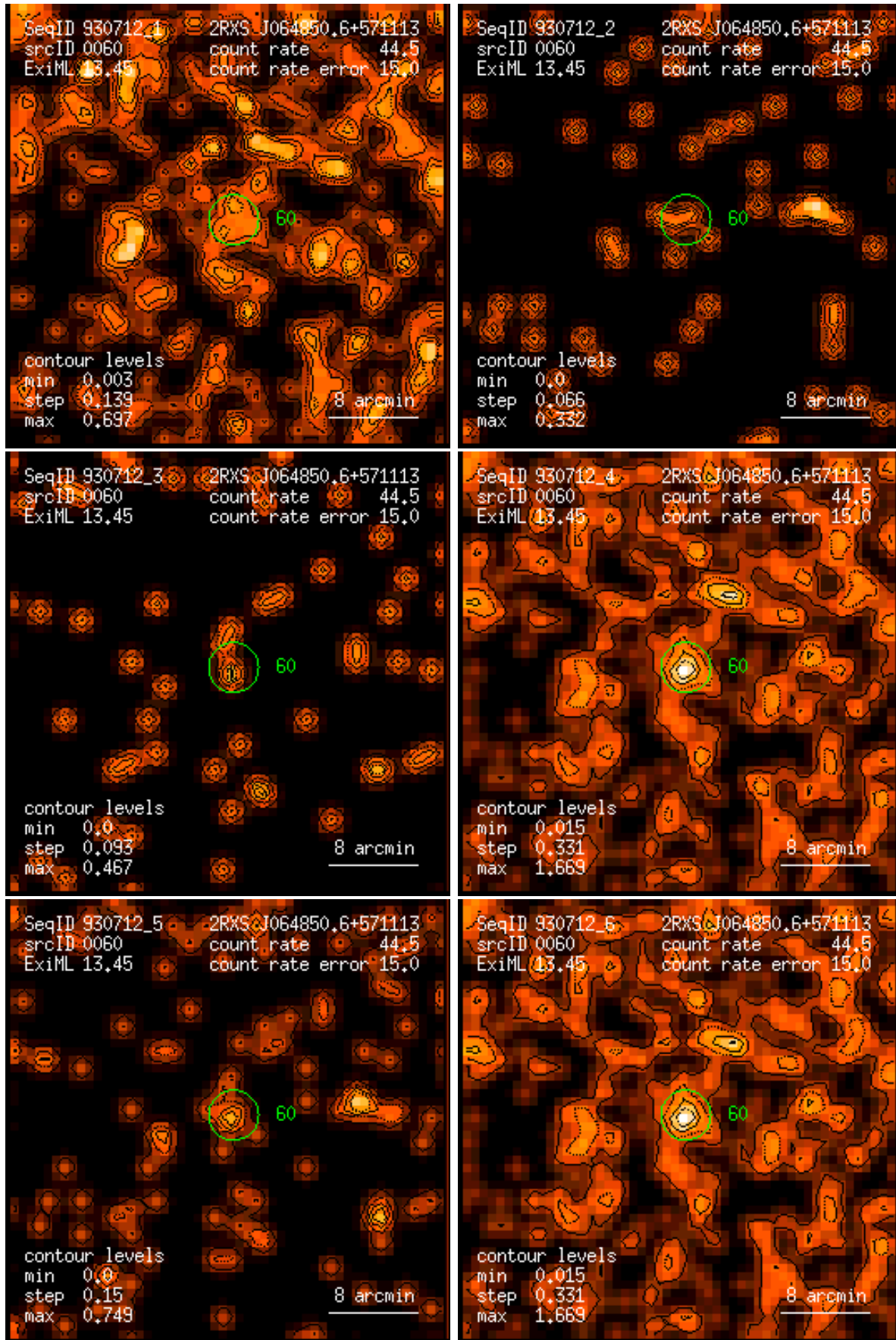
Figure 60: RASS 930712: detection 0060: band rate images, Gaussian filter: (1) PSPC channels 11 – 41, (2) 52 – 90, (3) 91 – 201, (4) 11 – 235, (5) 52 – 201, (6) 11 – 201. Broad band rates in counts/ks. Band rate contour levels in counts/ks/arcmin 2 .
