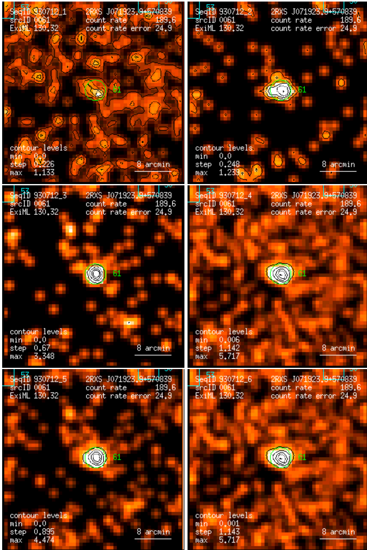
Figure 61: RASS 930712: detection 0061: band rate images, Gaussian filter: (1) PSPC channels 11 – 41, (2) 52 – 90, (3) 91 – 201, (4) 11 – 235, (5) 52 – 201, (6) 11 – 201. Broad band rates in counts/ks. Band rate contour levels in counts/ks/arcmin 2 .
