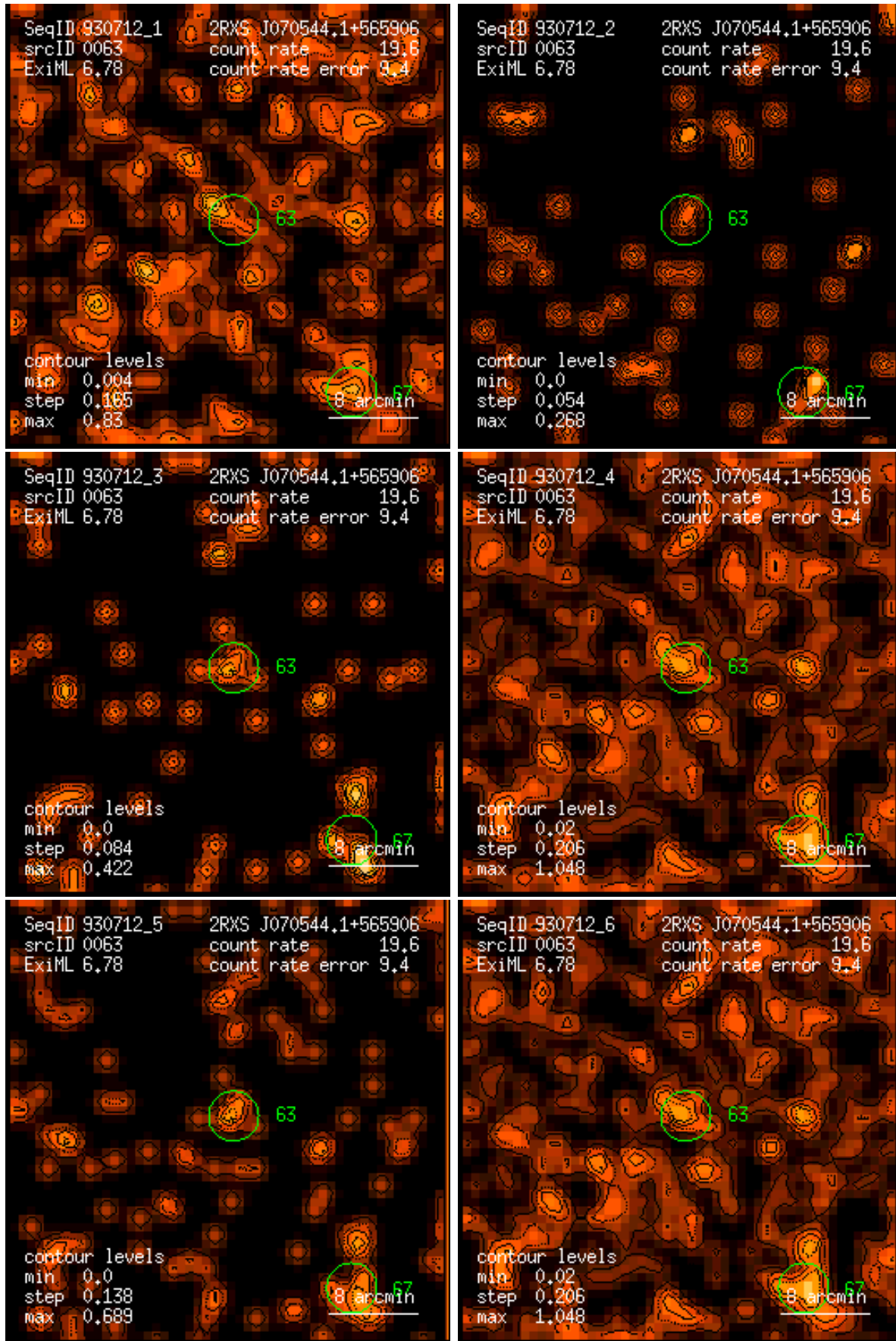
Figure 63: RASS 930712: detection 0063: band rate images, Gaussian filter: (1) PSPC channels 11 – 41, (2) 52 – 90, (3) 91 – 201, (4) 11 – 235, (5) 52 – 201, (6) 11 – 201. Broad band rates in counts/ks. Band rate contour levels in counts/ks/arcmin 2 .
