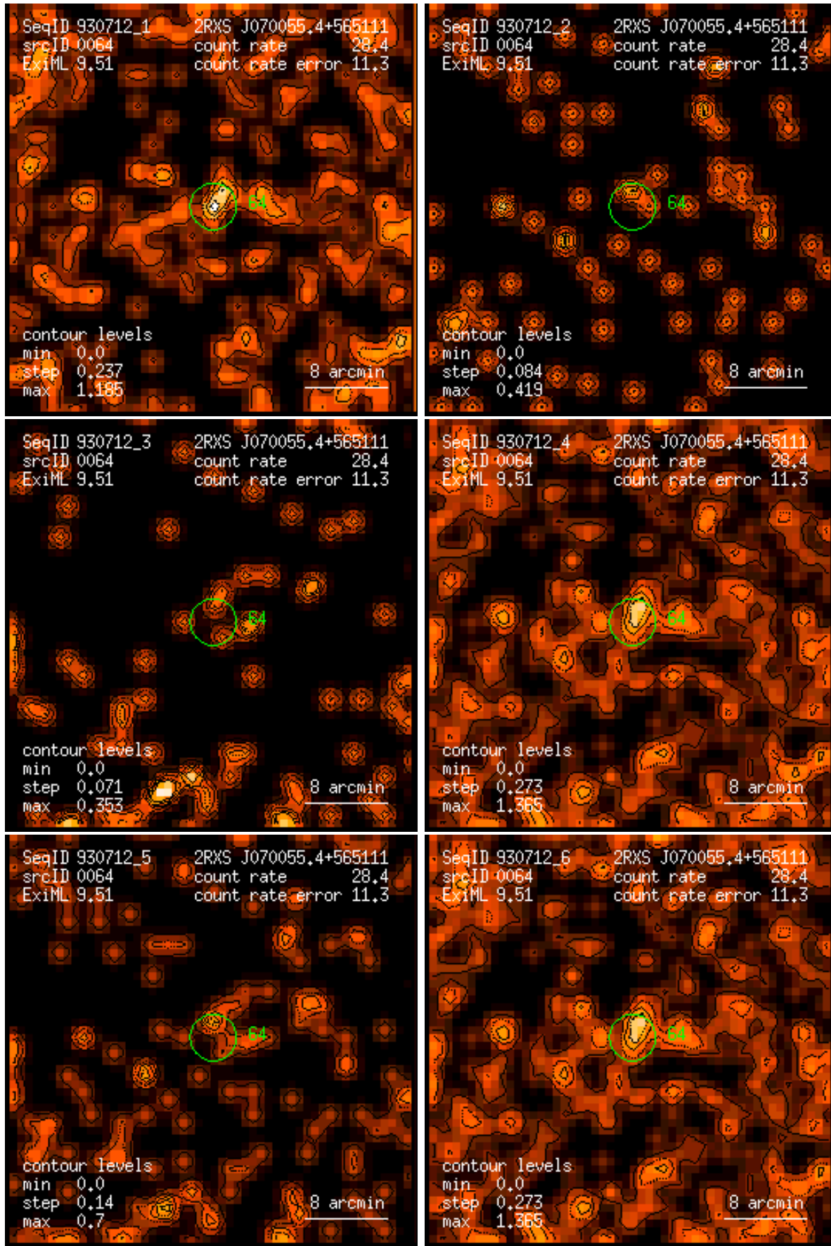
Figure 64: RASS 930712: detection 0064: band rate images, Gaussian filter: (1) PSPC channels 11 – 41, (2) 52 – 90, (3) 91 – 201, (4) 11 – 235, (5) 52 – 201, (6) 11 – 201. Broad band rates in counts/ks. Band rate contour levels in counts/ks/arcmin 2 .
