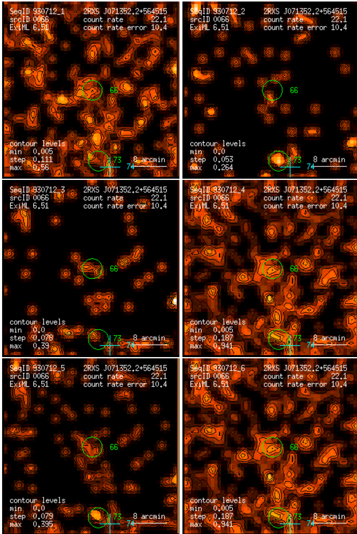
Figure 66: RASS 930712: detection 0066: band rate images, Gaussian filter: (1) PSPC channels 11 – 41, (2) 52 – 90, (3) 91 – 201, (4) 11 – 235, (5) 52 – 201, (6) 11 – 201. Broad band rates in counts/ks. Band rate contour levels in counts/ks/arcmin 2 .
