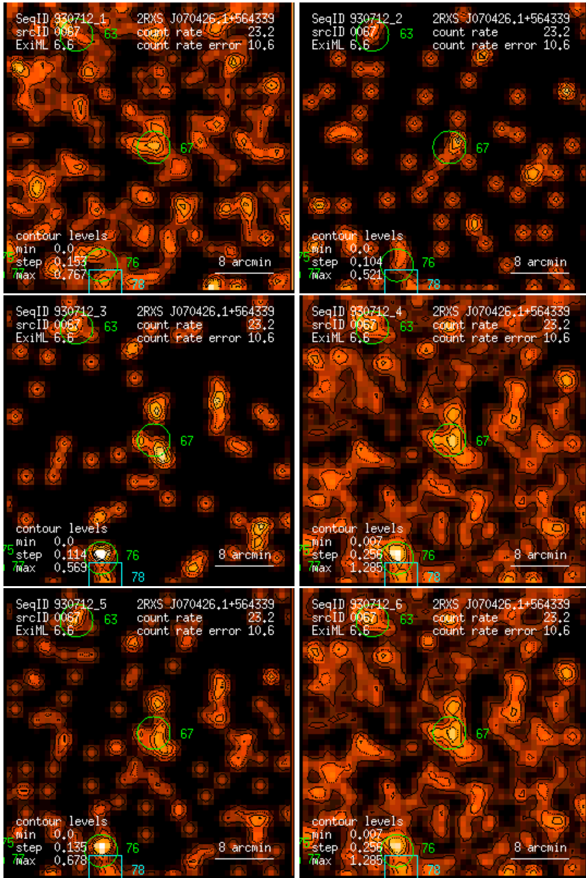
Figure 67: RASS 930712: detection 0067: band rate images, Gaussian filter: (1) PSPC channels 11 – 41, (2) 52 – 90, (3) 91 – 201, (4) 11 – 235, (5) 52 – 201, (6) 11 – 201. Broad band rates in counts/ks. Band rate contour levels in counts/ks/arcmin 2 .
