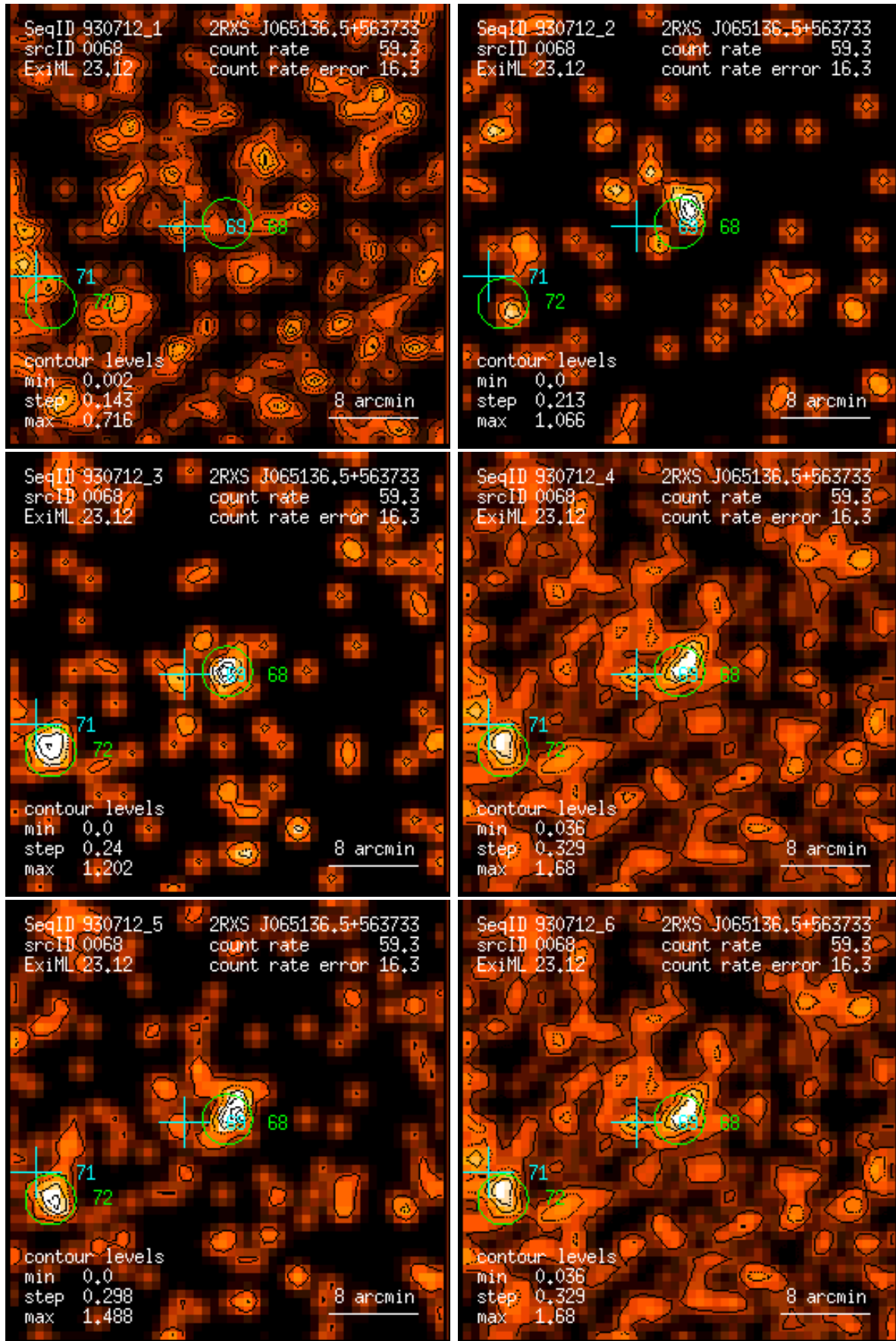
Figure 68: RASS 930712: detection 0068: band rate images, Gaussian filter: (1) PSPC channels 11 – 41, (2) 52 – 90, (3) 91 – 201, (4) 11 – 235, (5) 52 – 201, (6) 11 – 201. Broad band rates in counts/ks. Band rate contour levels in counts/ks/arcmin 2 .
