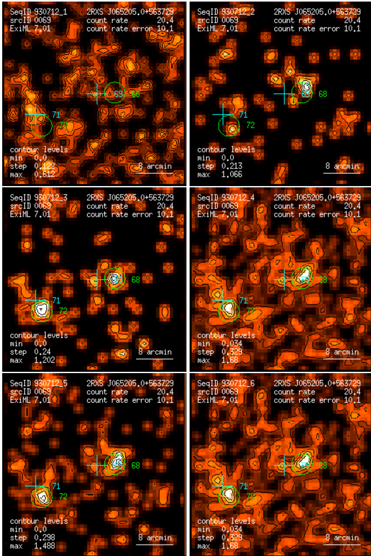
Figure 69: RASS 930712: detection 0069: band rate images, Gaussian filter: (1) PSPC channels 11 – 41, (2) 52 – 90, (3) 91 – 201, (4) 11 – 235, (5) 52 – 201, (6) 11 – 201. Broad band rates in counts/ks. Band rate contour levels in counts/ks/arcmin 2 .
