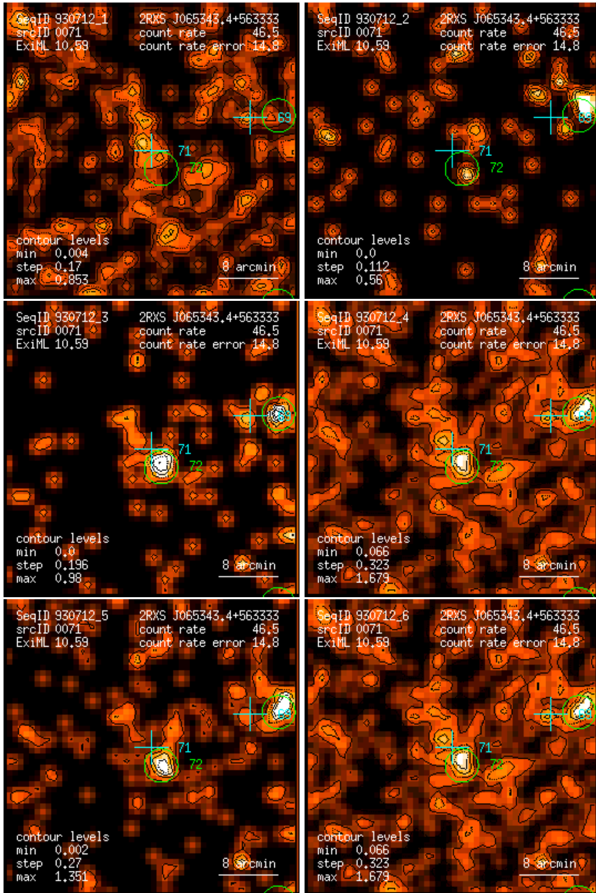
Figure 71: RASS 930712: detection 0071: band rate images, Gaussian filter: (1) PSPC channels 11 – 41, (2) 52 – 90, (3) 91 – 201, (4) 11 – 235, (5) 52 – 201, (6) 11 – 201. Broad band rates in counts/ks. Band rate contour levels in counts/ks/arcmin 2 .
