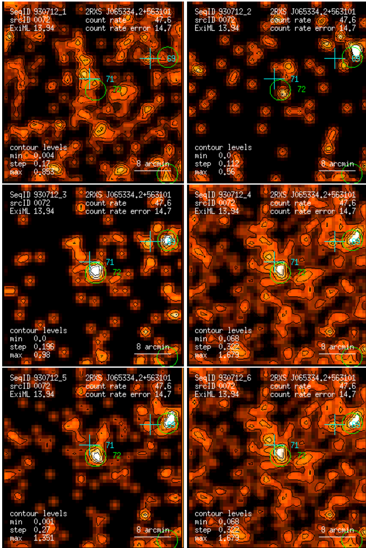
Figure 72: RASS 930712: detection 0072: band rate images, Gaussian filter: (1) PSPC channels 11 – 41, (2) 52 – 90, (3) 91 – 201, (4) 11 – 235, (5) 52 – 201, (6) 11 – 201. Broad band rates in counts/ks. Band rate contour levels in counts/ks/arcmin 2 .
