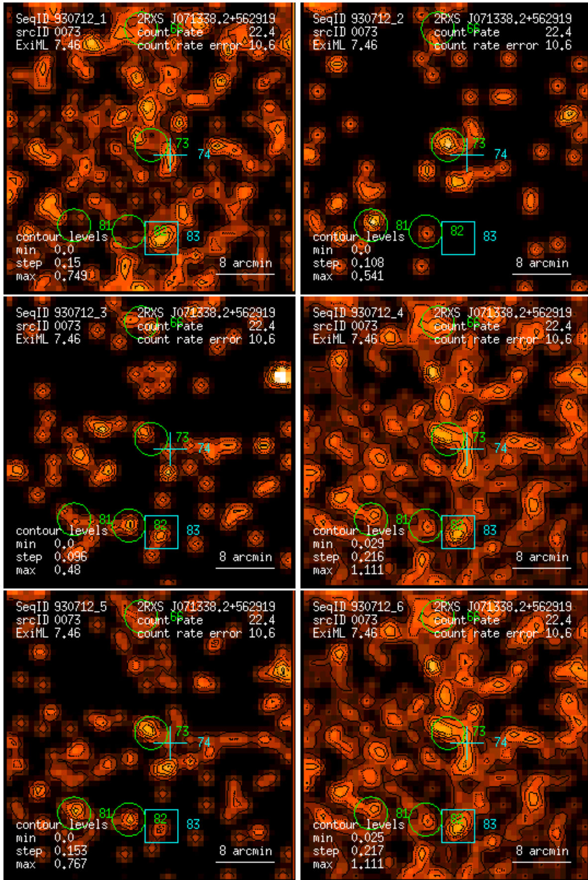
Figure 73: RASS 930712: detection 0073: band rate images, Gaussian filter: (1) PSPC channels 11 – 41, (2) 52 – 90, (3) 91 – 201, (4) 11 – 235, (5) 52 – 201, (6) 11 – 201. Broad band rates in counts/ks. Band rate contour levels in counts/ks/arcmin 2 .
