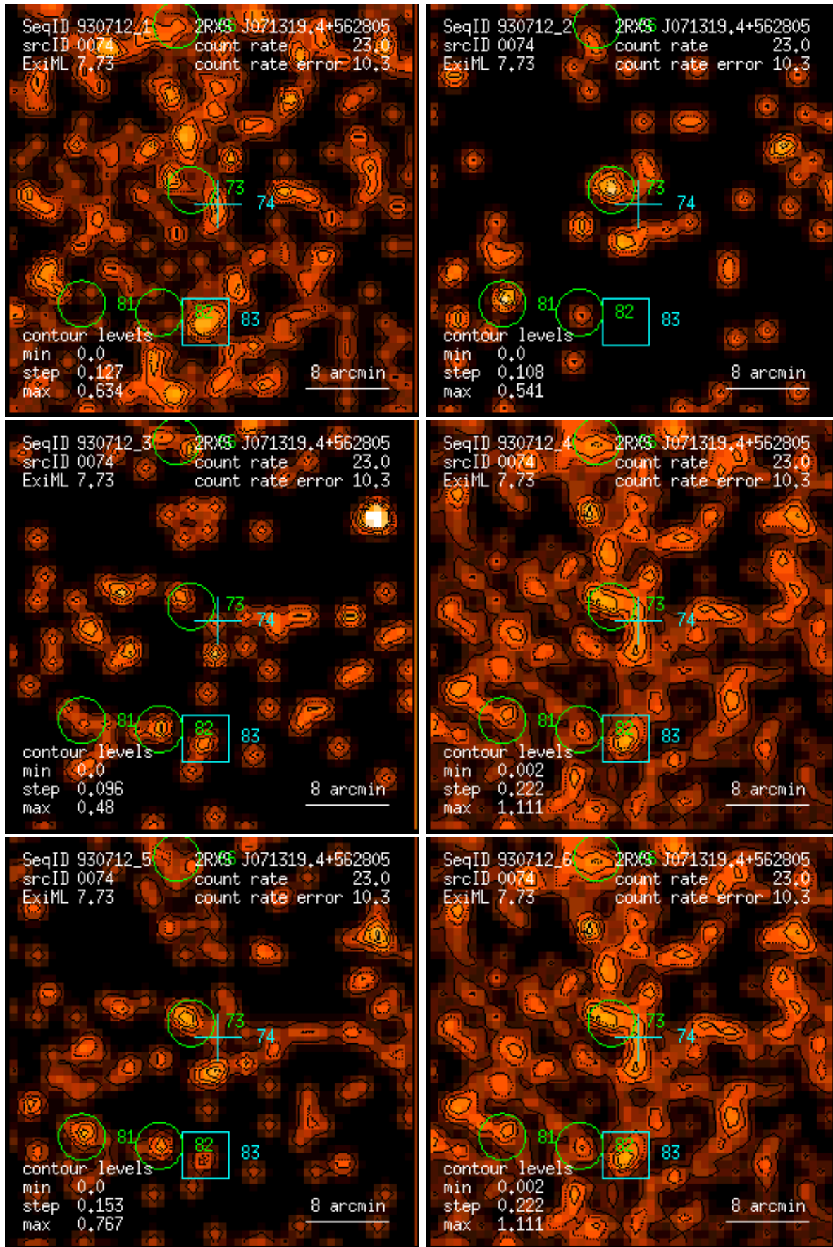
Figure 74: RASS 930712: detection 0074: band rate images, Gaussian filter: (1) PSPC channels 11 – 41, (2) 52 – 90, (3) 91 – 201, (4) 11 – 235, (5) 52 – 201, (6) 11 – 201. Broad band rates in counts/ks. Band rate contour levels in counts/ks/arcmin 2 .
