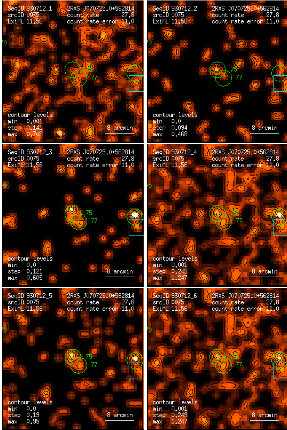
Figure 75: RASS 930712: detection 0075: band rate images, Gaussian filter: (1) PSPC channels 11 – 41, (2) 52 – 90, (3) 91 – 201, (4) 11 – 235, (5) 52 – 201, (6) 11 – 201. Broad band rates in counts/ks. Band rate contour levels in counts/ks/arcmin 2 .
