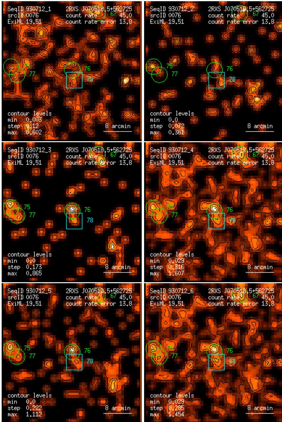
Figure 76: RASS 930712: detection 0076: band rate images, Gaussian filter: (1) PSPC channels 11 – 41, (2) 52 – 90, (3) 91 – 201, (4) 11 – 235, (5) 52 – 201, (6) 11 – 201. Broad band rates in counts/ks. Band rate contour levels in counts/ks/arcmin 2 .
