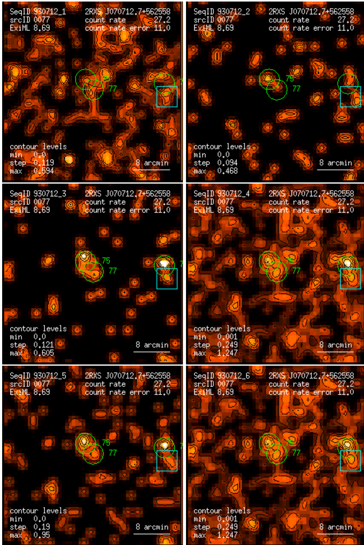
Figure 77: RASS 930712: detection 0077: band rate images, Gaussian filter: (1) PSPC channels 11 – 41, (2) 52 – 90, (3) 91 – 201, (4) 11 – 235, (5) 52 – 201, (6) 11 – 201. Broad band rates in counts/ks. Band rate contour levels in counts/ks/arcmin 2 .
