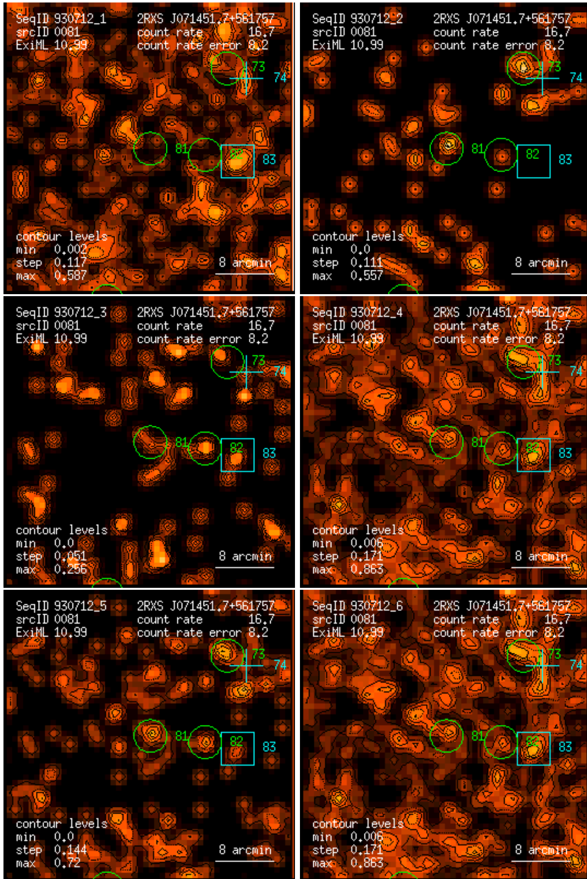
Figure 81: RASS 930712: detection 0081: band rate images, Gaussian filter: (1) PSPC channels 11 – 41, (2) 52 – 90, (3) 91 – 201, (4) 11 – 235, (5) 52 – 201, (6) 11 – 201. Broad band rates in counts/ks. Band rate contour levels in counts/ks/arcmin 2 .
