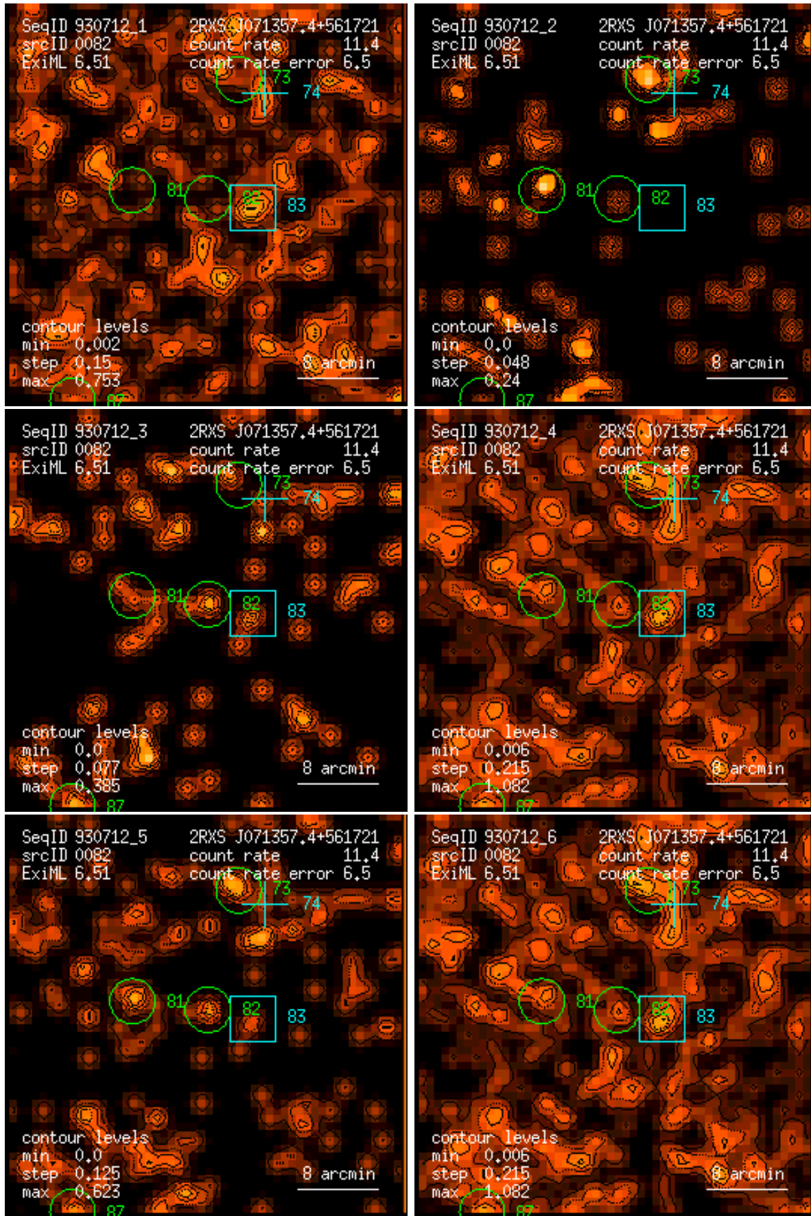
Figure 82: RASS 930712: detection 0082: band rate images, Gaussian filter: (1) PSPC channels 11 – 41, (2) 52 – 90, (3) 91 – 201, (4) 11 – 235, (5) 52 – 201, (6) 11 – 201. Broad band rates in counts/ks. Band rate contour levels in counts/ks/arcmin 2 .
