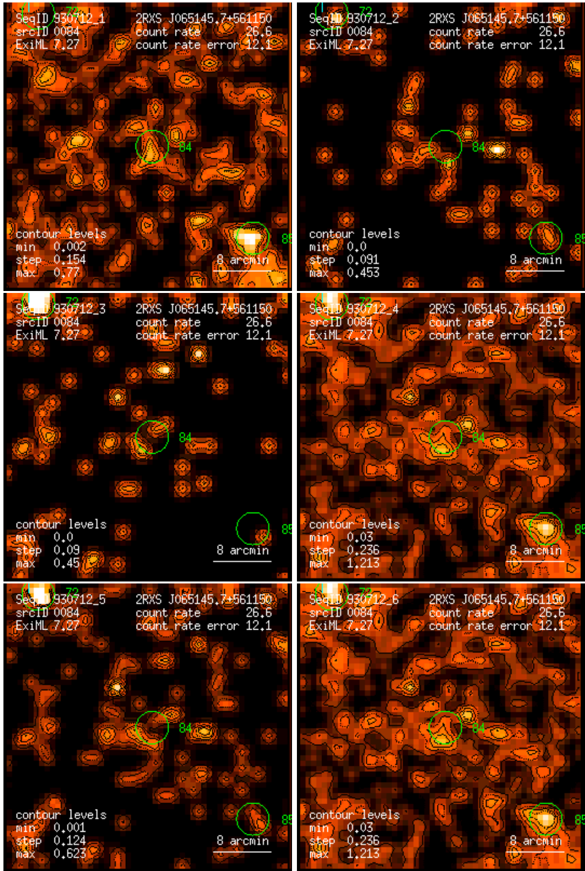
Figure 84: RASS 930712: detection 0084: band rate images, Gaussian filter: (1) PSPC channels 11 – 41, (2) 52 – 90, (3) 91 – 201, (4) 11 – 235, (5) 52 – 201, (6) 11 – 201. Broad band rates in counts/ks. Band rate contour levels in counts/ks/arcmin 2 .
