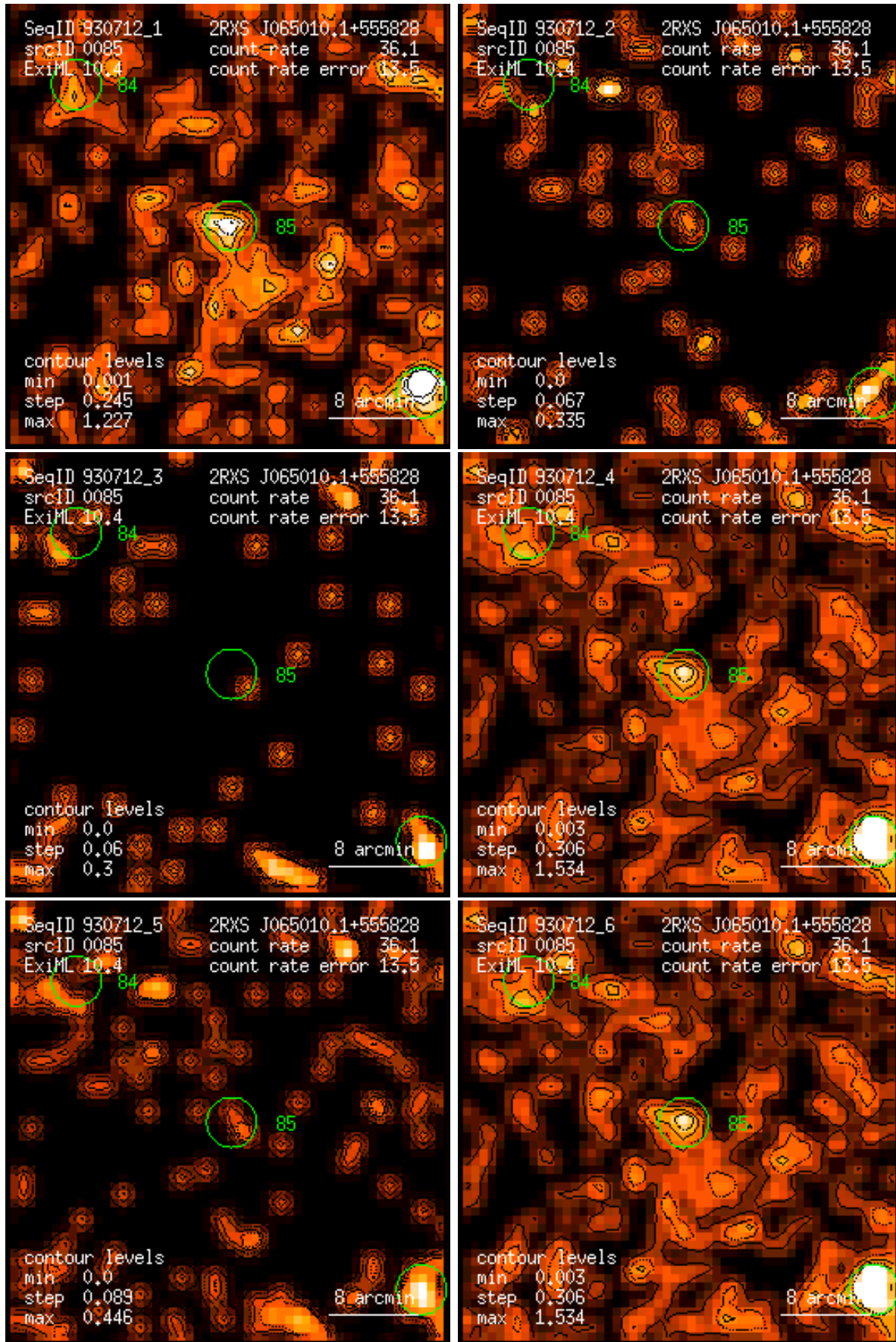
Figure 85: RASS 930712: detection 0085: band rate images, Gaussian filter: (1) PSPC channels 11 – 41, (2) 52 – 90, (3) 91 – 201, (4) 11 – 235, (5) 52 – 201, (6) 11 – 201. Broad band rates in counts/ks. Band rate contour levels in counts/ks/arcmin 2 .
