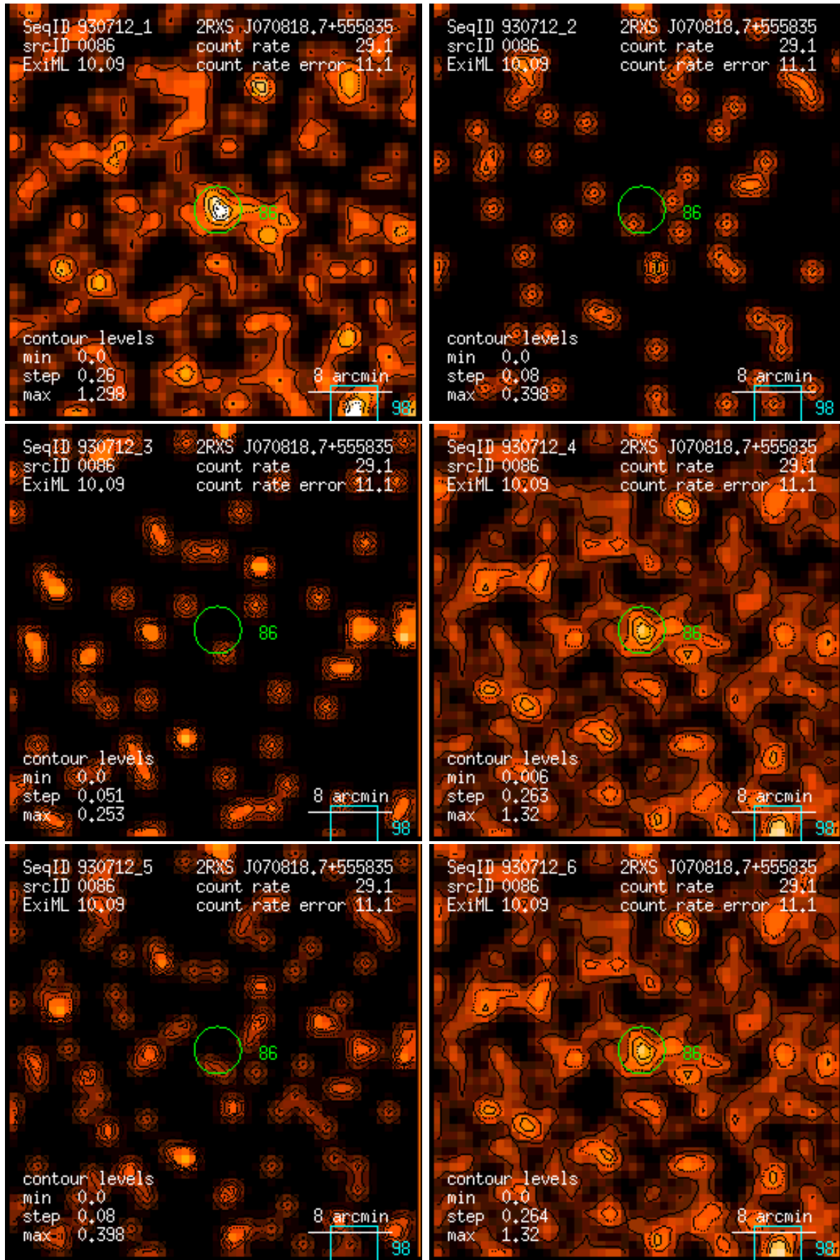
Figure 86: RASS 930712: detection 0086: band rate images, Gaussian filter: (1) PSPC channels 11 – 41, (2) 52 – 90, (3) 91 – 201, (4) 11 – 235, (5) 52 – 201, (6) 11 – 201. Broad band rates in counts/ks. Band rate contour levels in counts/ks/arcmin 2 .
