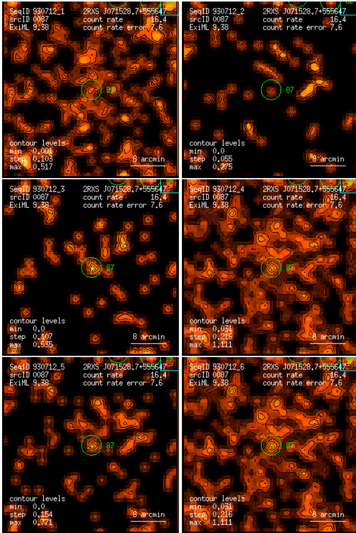
Figure 87: RASS 930712: detection 0087: band rate images, Gaussian filter: (1) PSPC channels 11 – 41, (2) 52 – 90, (3) 91 – 201, (4) 11 – 235, (5) 52 – 201, (6) 11 – 201. Broad band rates in counts/ks. Band rate contour levels in counts/ks/arcmin 2 .
