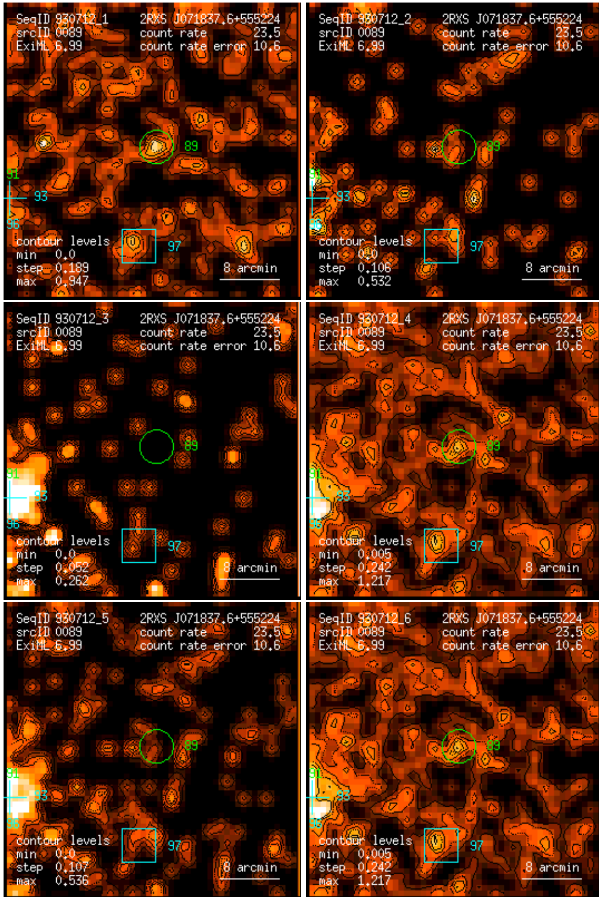
Figure 89: RASS 930712: detection 0089: band rate images, Gaussian filter: (1) PSPC channels 11 – 41, (2) 52 – 90, (3) 91 – 201, (4) 11 – 235, (5) 52 – 201, (6) 11 – 201. Broad band rates in counts/ks. Band rate contour levels in counts/ks/arcmin 2 .
