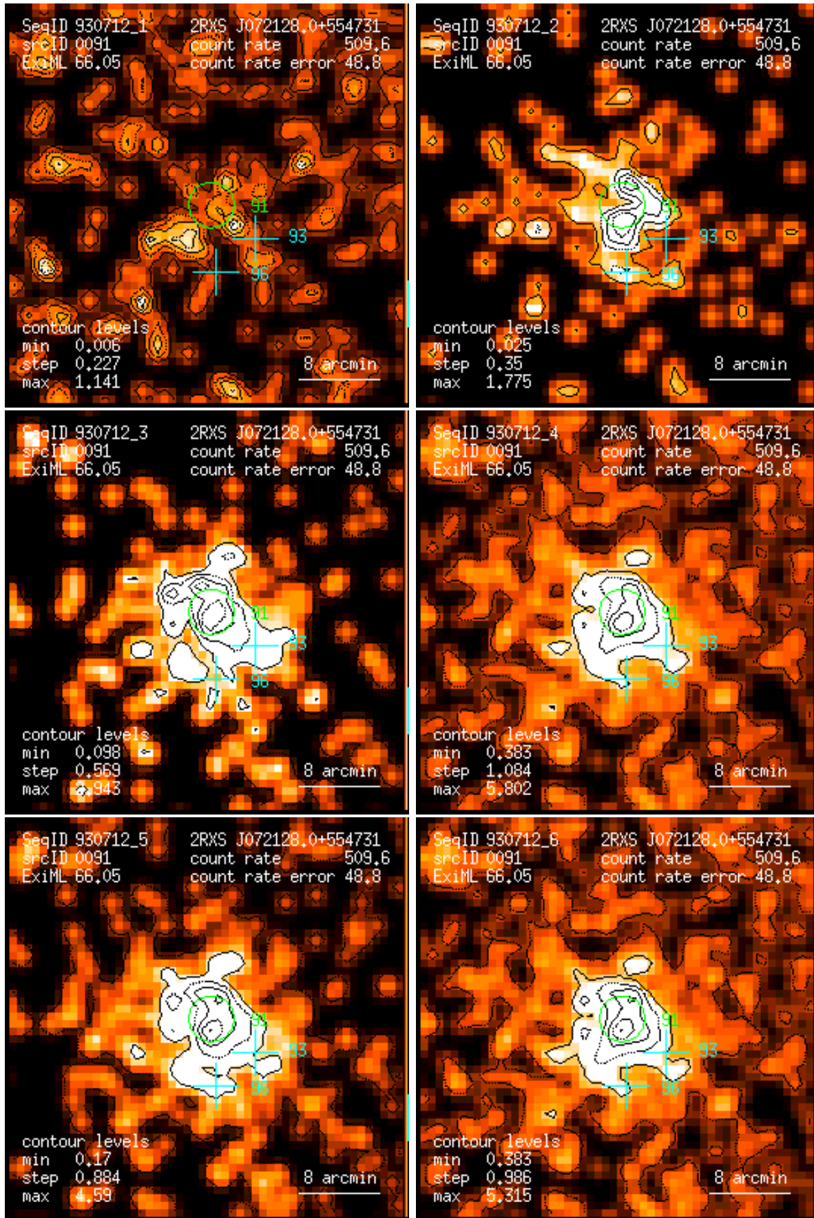
Figure 91: RASS 930712: detection 0091: band rate images, Gaussian filter: (1) PSPC channels 11 – 41, (2) 52 – 90, (3) 91 – 201, (4) 11 – 235, (5) 52 – 201, (6) 11 – 201. Broad band rates in counts/ks. Band rate contour levels in counts/ks/arcmin 2 .
