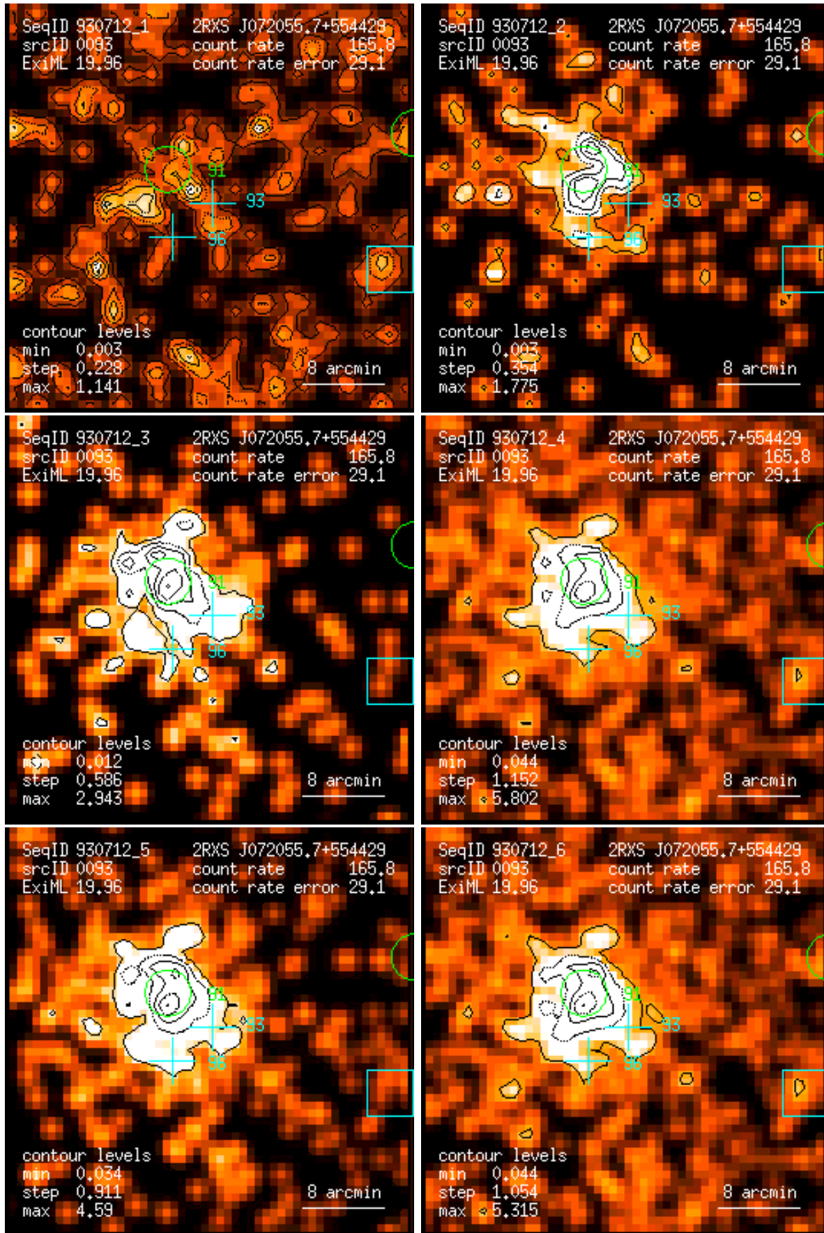
Figure 93: RASS 930712: detection 0093: band rate images, Gaussian filter: (1) PSPC channels 11 – 41, (2) 52 – 90, (3) 91 – 201, (4) 11 – 235, (5) 52 – 201, (6) 11 – 201. Broad band rates in counts/ks. Band rate contour levels in counts/ks/arcmin 2 .
