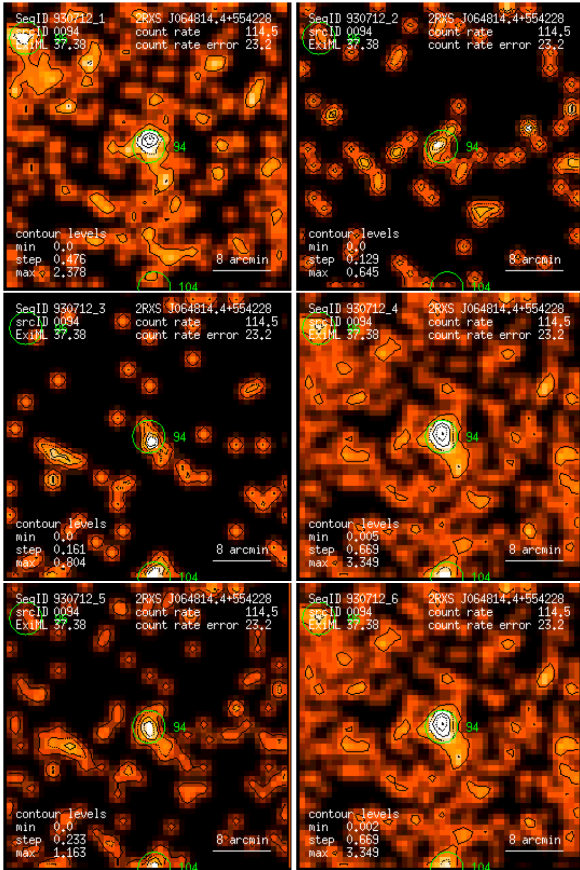
Figure 94: RASS 930712: detection 0094: band rate images, Gaussian filter: (1) PSPC channels 11 – 41, (2) 52 – 90, (3) 91 – 201, (4) 11 – 235, (5) 52 – 201, (6) 11 – 201. Broad band rates in counts/ks. Band rate contour levels in counts/ks/arcmin 2 .
