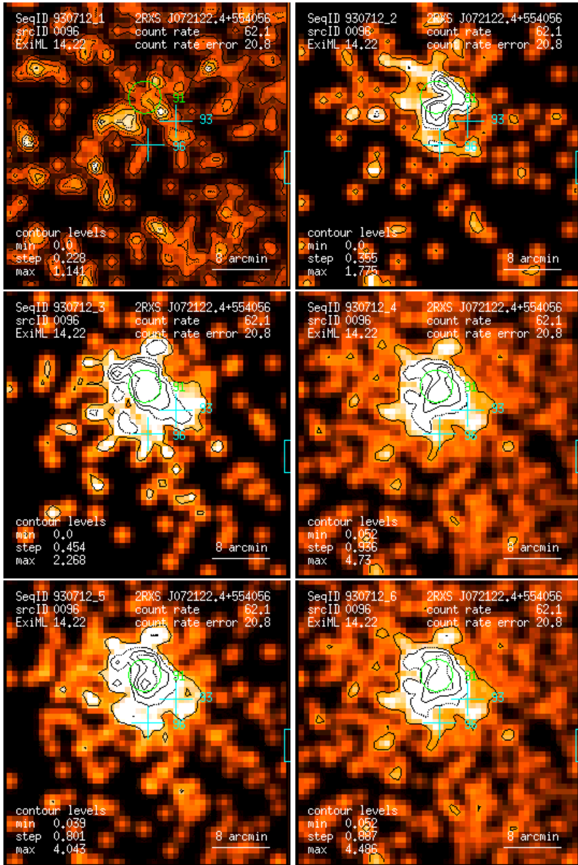
Figure 96: RASS 930712: detection 0096: band rate images, Gaussian filter: (1) PSPC channels 11 – 41, (2) 52 – 90, (3) 91 – 201, (4) 11 – 235, (5) 52 – 201, (6) 11 – 201. Broad band rates in counts/ks. Band rate contour levels in counts/ks/arcmin 2 .
