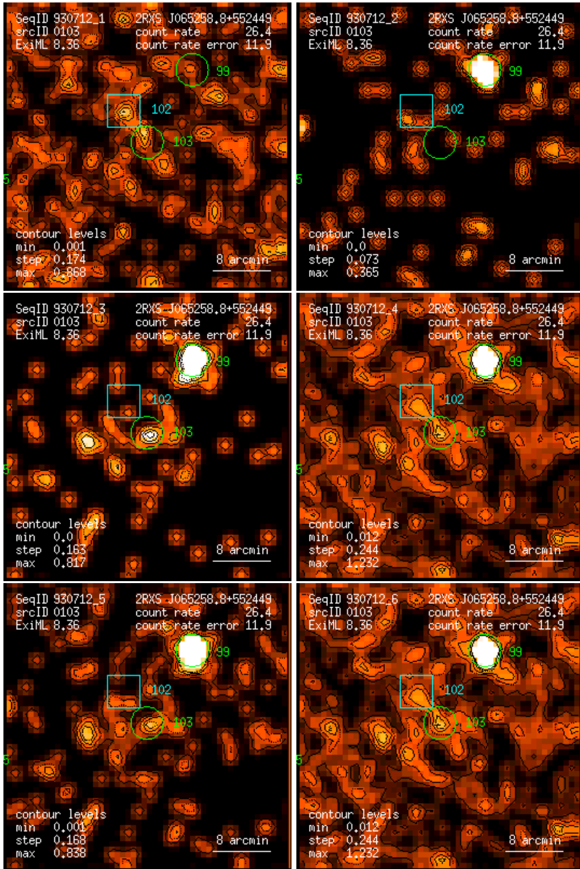
Figure 103: RASS 930712: detection 0103: band rate images, Gaussian filter: (1) PSPC channels 11 – 41, (2) 52 – 90, (3) 91 – 201, (4) 11 – 235, (5) 52 – 201, (6) 11 – 201. Broad band rates in counts/ks. Band rate contour levels in counts/ks/arcmin 2 .
