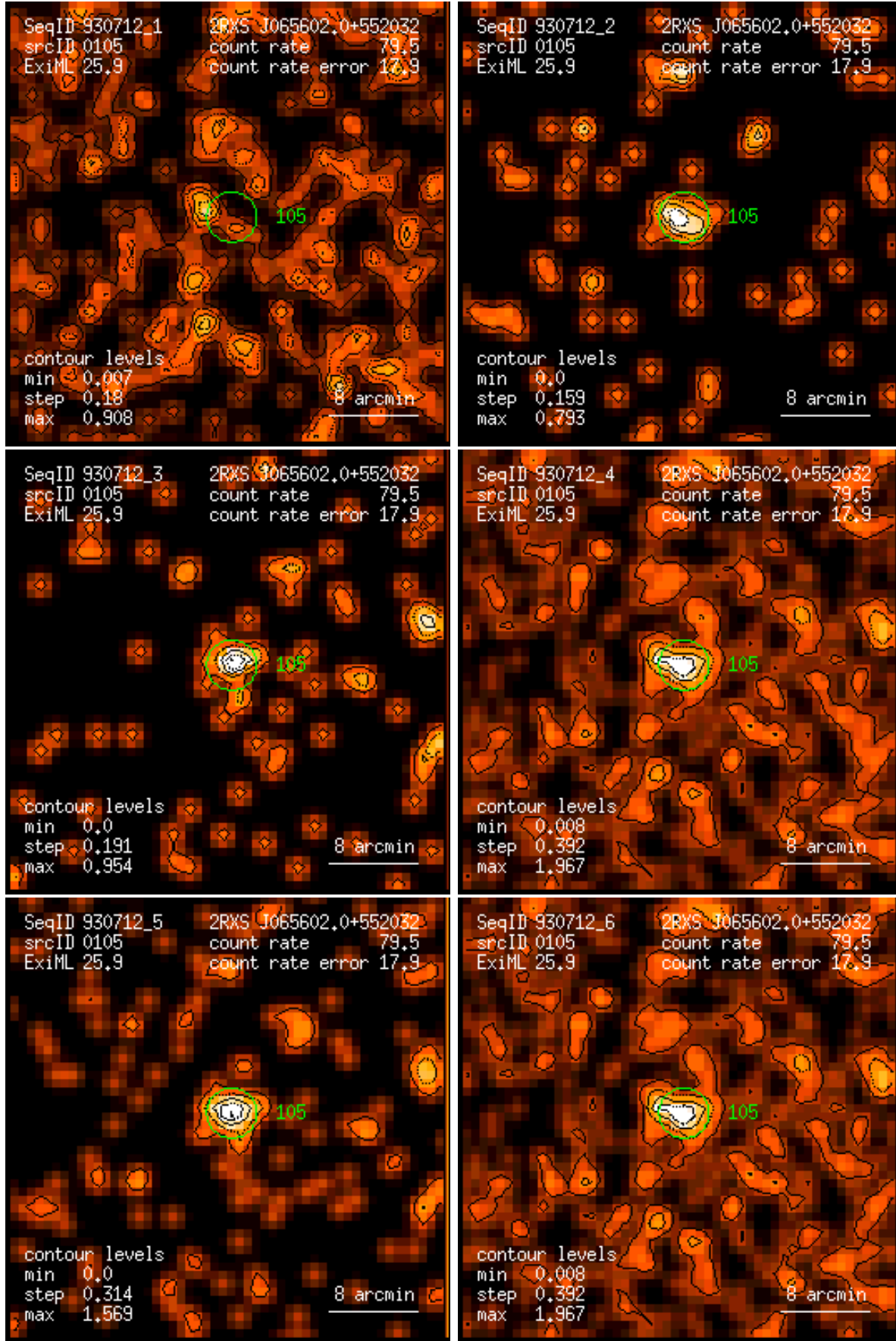
Figure 105: RASS 930712: detection 0105: band rate images, Gaussian filter: (1) PSPC channels 11 – 41, (2) 52 – 90, (3) 91 – 201, (4) 11 – 235, (5) 52 – 201, (6) 11 – 201. Broad band rates in counts/ks. Band rate contour levels in counts/ks/arcmin 2 .
