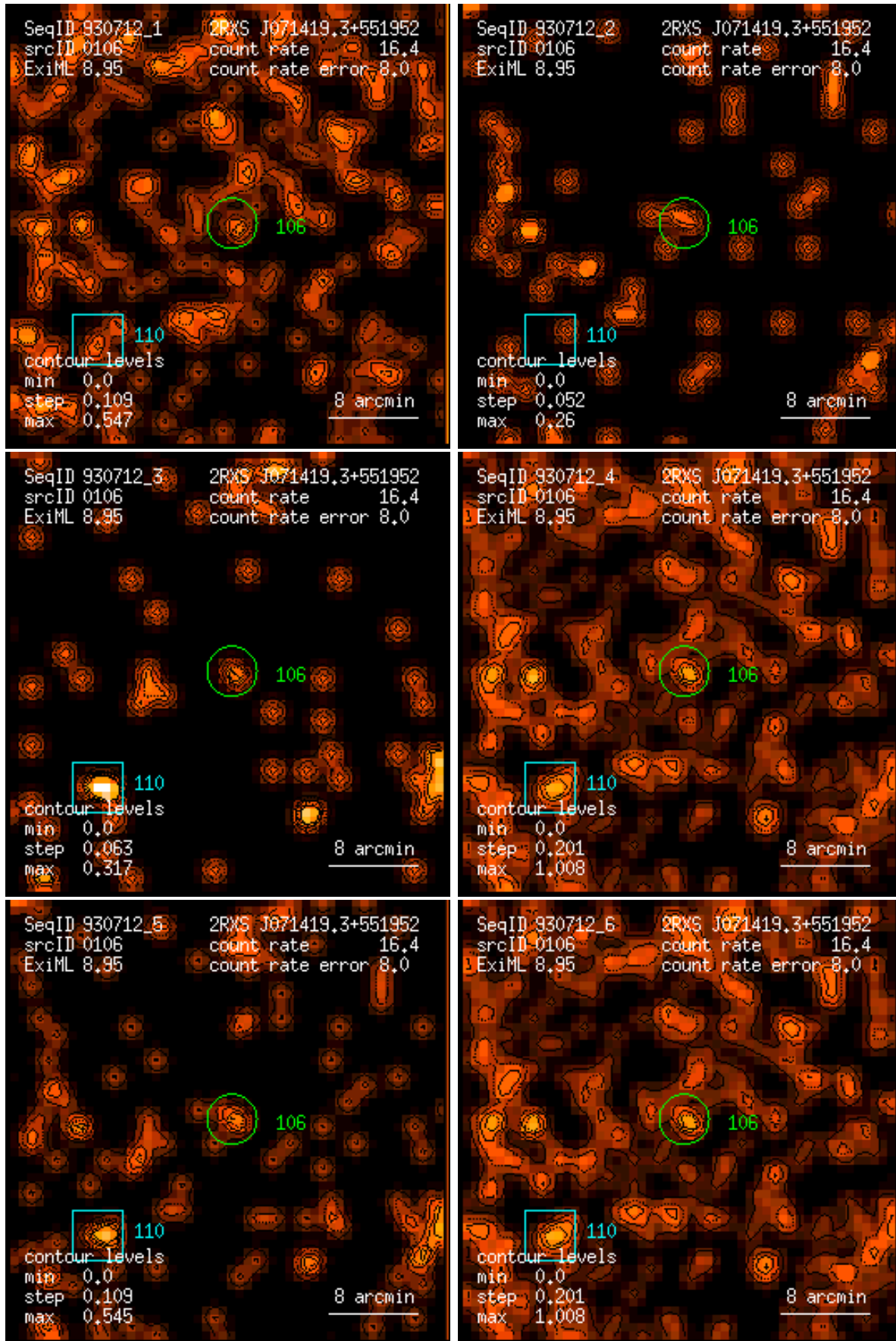
Figure 106: RASS 930712: detection 0106: band rate images, Gaussian filter: (1) PSPC channels 11 – 41, (2) 52 – 90, (3) 91 – 201, (4) 11 – 235, (5) 52 – 201, (6) 11 – 201. Broad band rates in counts/ks. Band rate contour levels in counts/ks/arcmin 2 .
