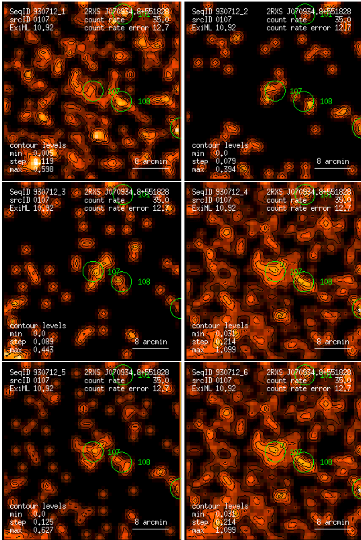
Figure 107: RASS 930712: detection 0107: band rate images, Gaussian filter: (1) PSPC channels 11 – 41, (2) 52 – 90, (3) 91 – 201, (4) 11 – 235, (5) 52 – 201, (6) 11 – 201. Broad band rates in counts/ks. Band rate contour levels in counts/ks/arcmin 2 .
