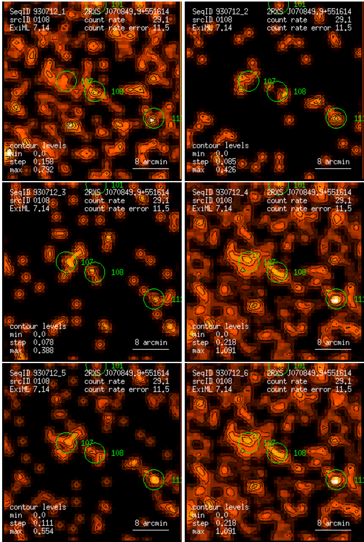
Figure 108: RASS 930712: detection 0108: band rate images, Gaussian filter: (1) PSPC channels 11 – 41, (2) 52 – 90, (3) 91 – 201, (4) 11 – 235, (5) 52 – 201, (6) 11 – 201. Broad band rates in counts/ks. Band rate contour levels in counts/ks/arcmin 2 .
