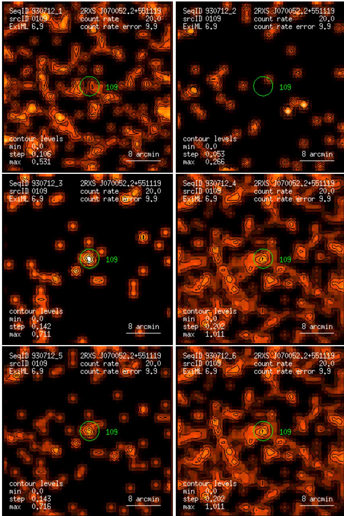
Figure 109: RASS 930712: detection 0109: band rate images, Gaussian filter: (1) PSPC channels 11 – 41, (2) 52 – 90, (3) 91 – 201, (4) 11 – 235, (5) 52 – 201, (6) 11 – 201. Broad band rates in counts/ks. Band rate contour levels in counts/ks/arcmin 2 .
