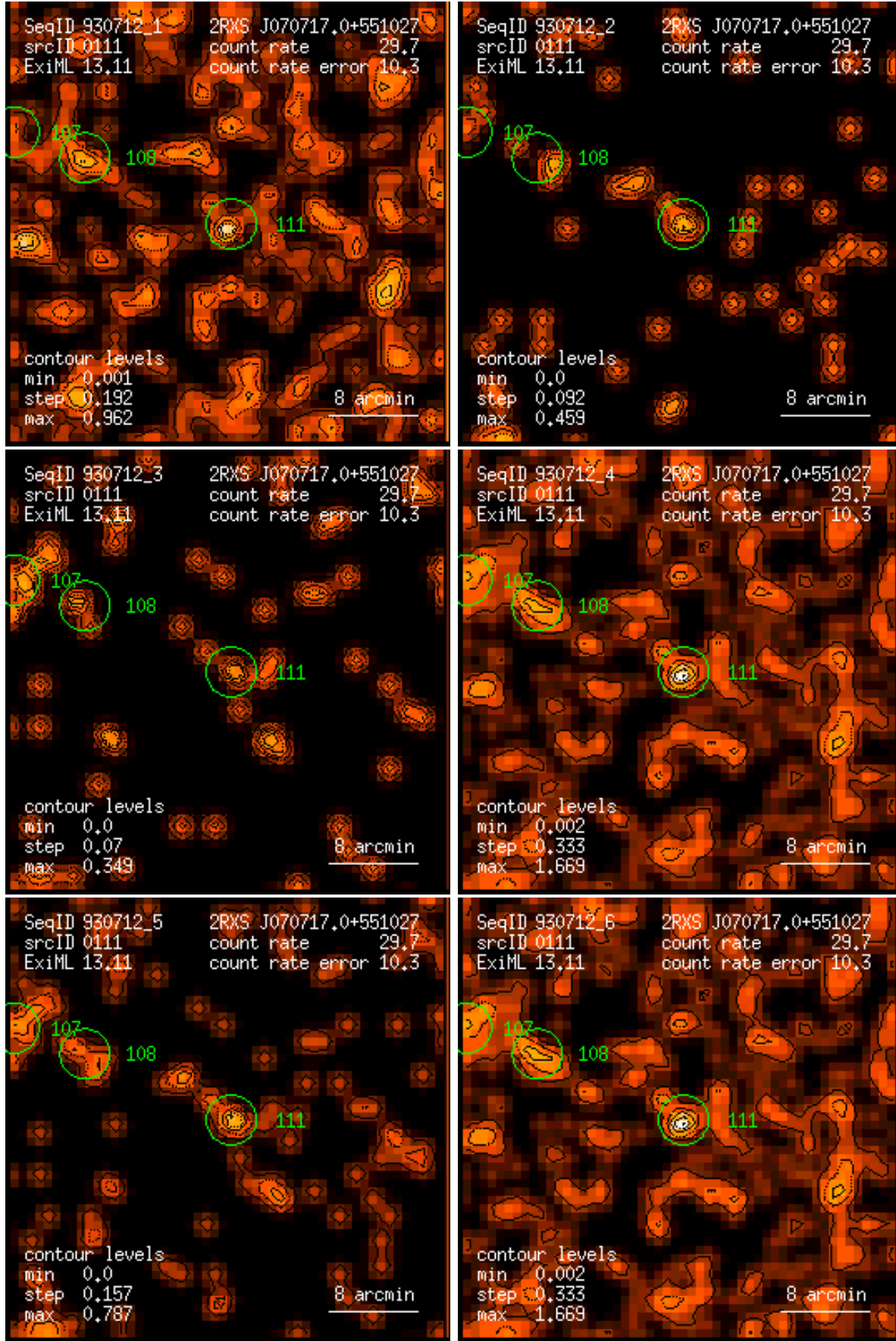
Figure 111: RASS 930712: detection 0111: band rate images, Gaussian filter: (1) PSPC channels 11 – 41, (2) 52 – 90, (3) 91 – 201, (4) 11 – 235, (5) 52 – 201, (6) 11 – 201. Broad band rates in counts/ks. Band rate contour levels in counts/ks/arcmin 2 .
