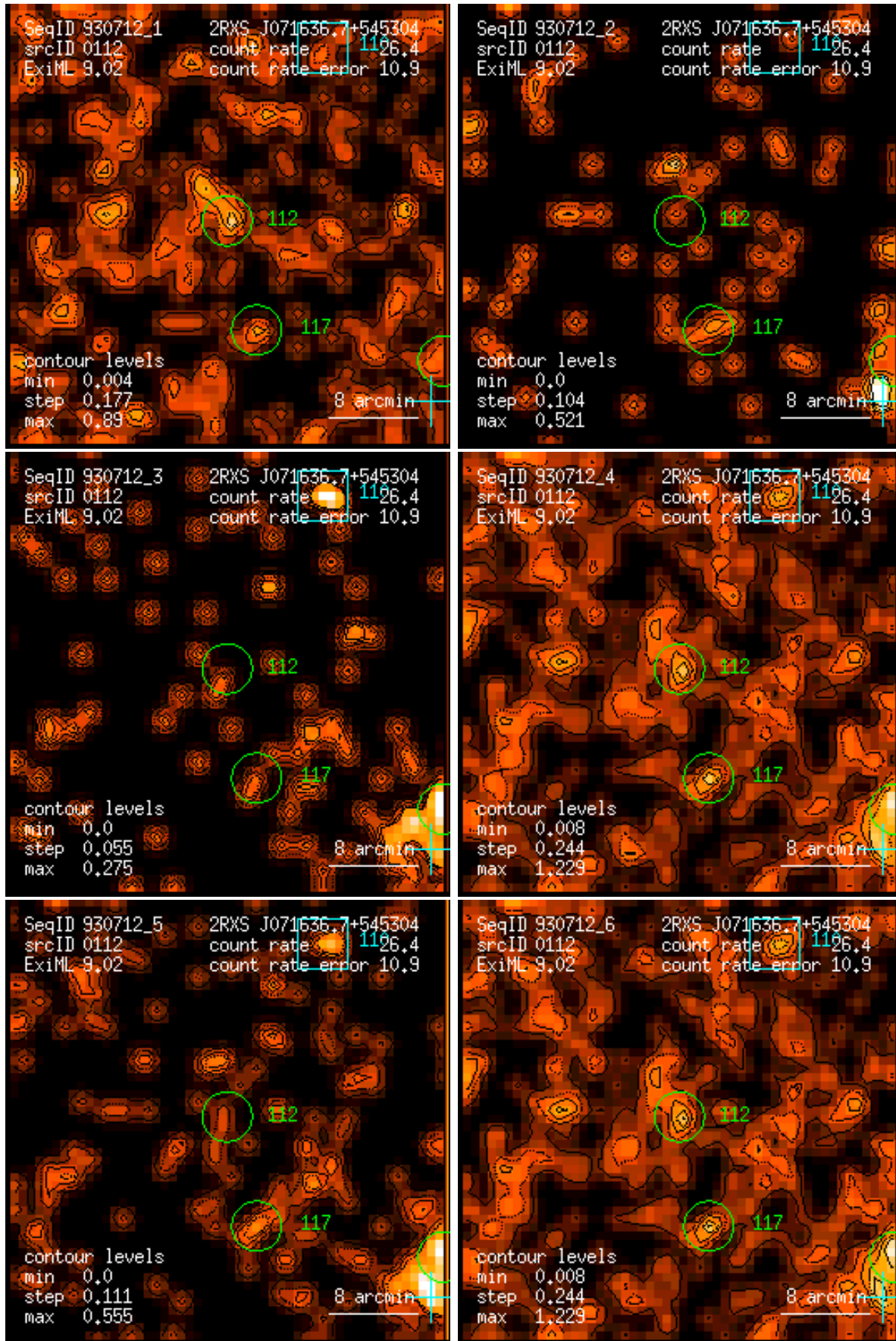
Figure 112: RASS 930712: detection 0112: band rate images, Gaussian filter: (1) PSPC channels 11 – 41, (2) 52 – 90, (3) 91 – 201, (4) 11 – 235, (5) 52 – 201, (6) 11 – 201. Broad band rates in counts/ks. Band rate contour levels in counts/ks/arcmin 2 .
