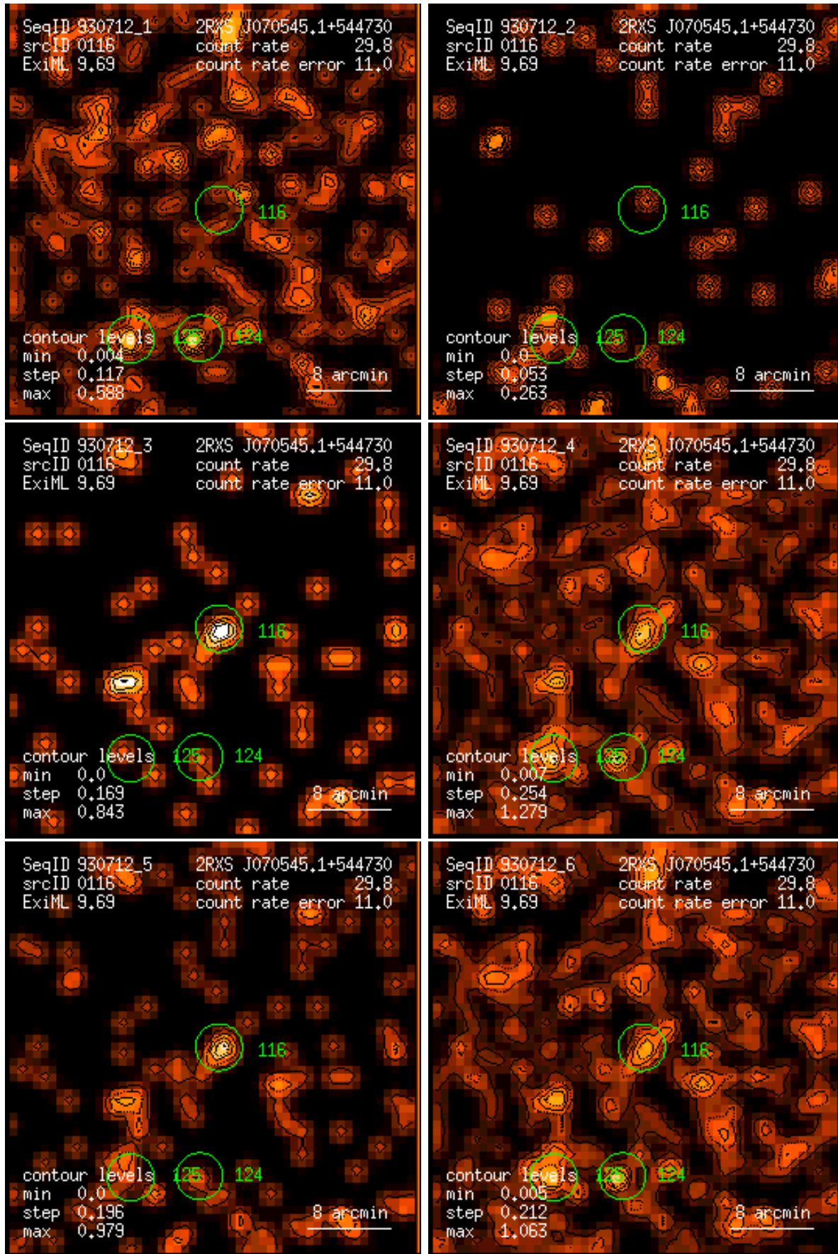
Figure 116: RASS 930712: detection 0116: band rate images, Gaussian filter: (1) PSPC channels 11 – 41, (2) 52 – 90, (3) 91 – 201, (4) 11 – 235, (5) 52 – 201, (6) 11 – 201. Broad band rates in counts/ks. Band rate contour levels in counts/ks/arcmin 2 .
