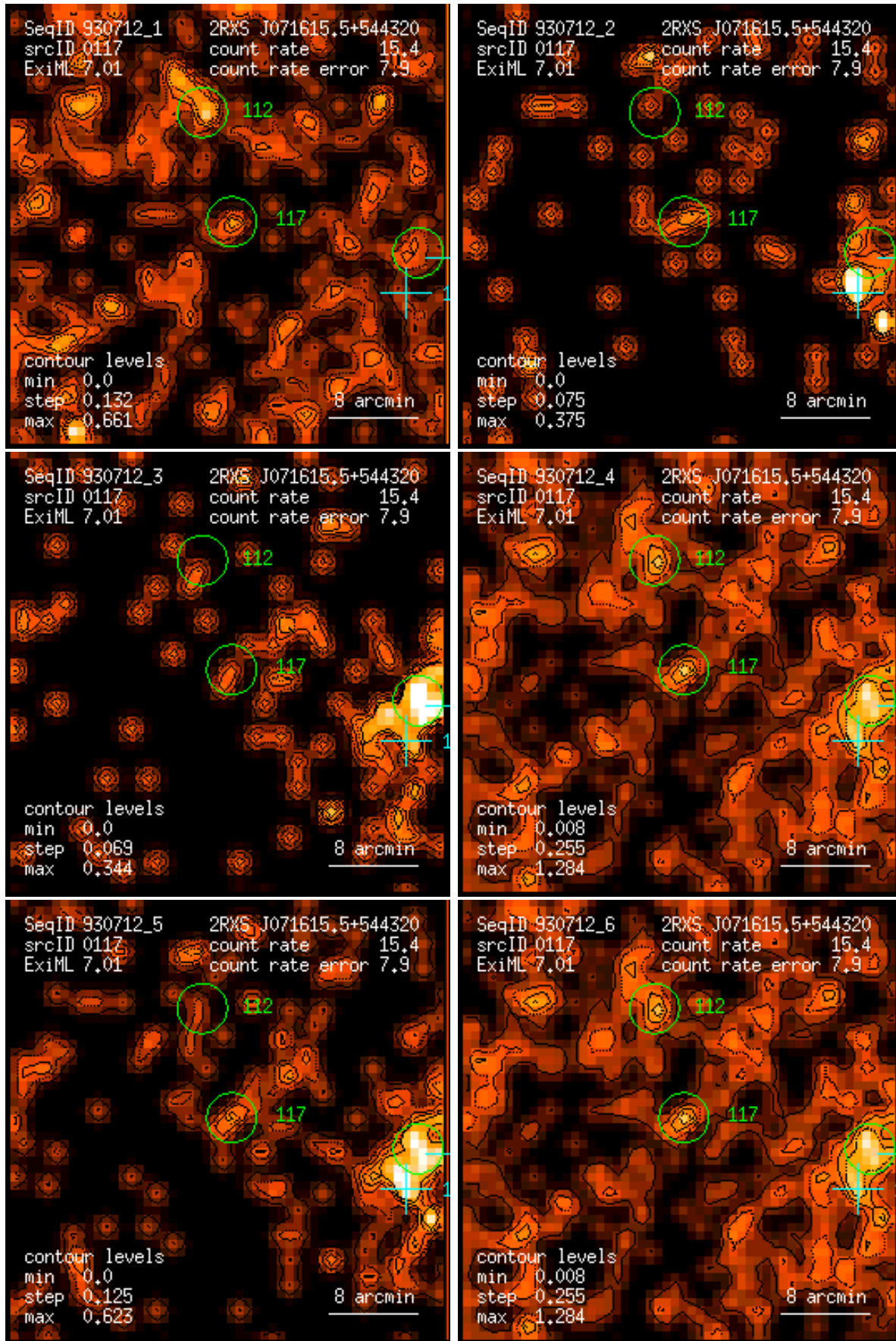
Figure 117: RASS 930712: detection 0117: band rate images, Gaussian filter: (1) PSPC channels 11 – 41, (2) 52 – 90, (3) 91 – 201, (4) 11 – 235, (5) 52 – 201, (6) 11 – 201. Broad band rates in counts/ks. Band rate contour levels in counts/ks/arcmin 2 .
