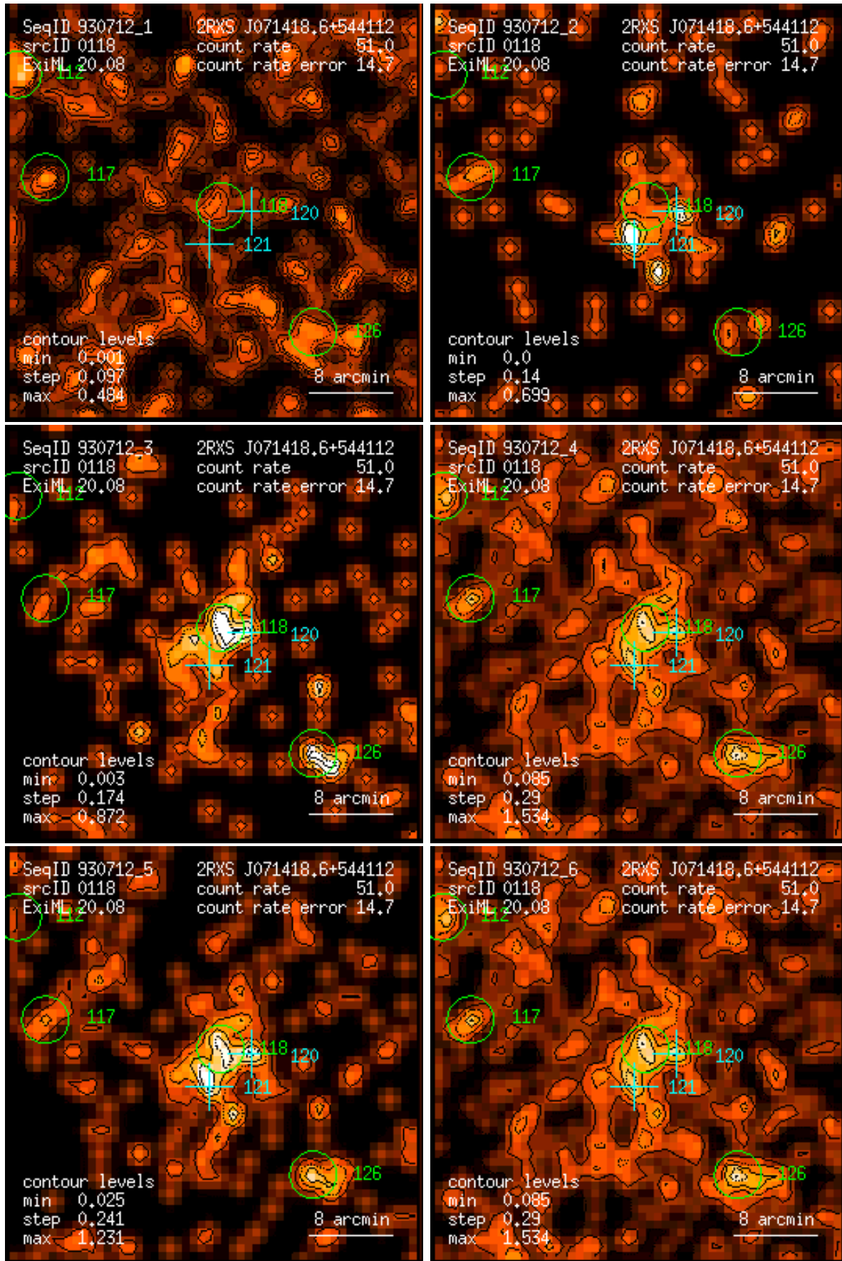
Figure 118: RASS 930712: detection 0118: band rate images, Gaussian filter: (1) PSPC channels 11 – 41, (2) 52 – 90, (3) 91 – 201, (4) 11 – 235, (5) 52 – 201, (6) 11 – 201. Broad band rates in counts/ks. Band rate contour levels in counts/ks/arcmin 2 .
