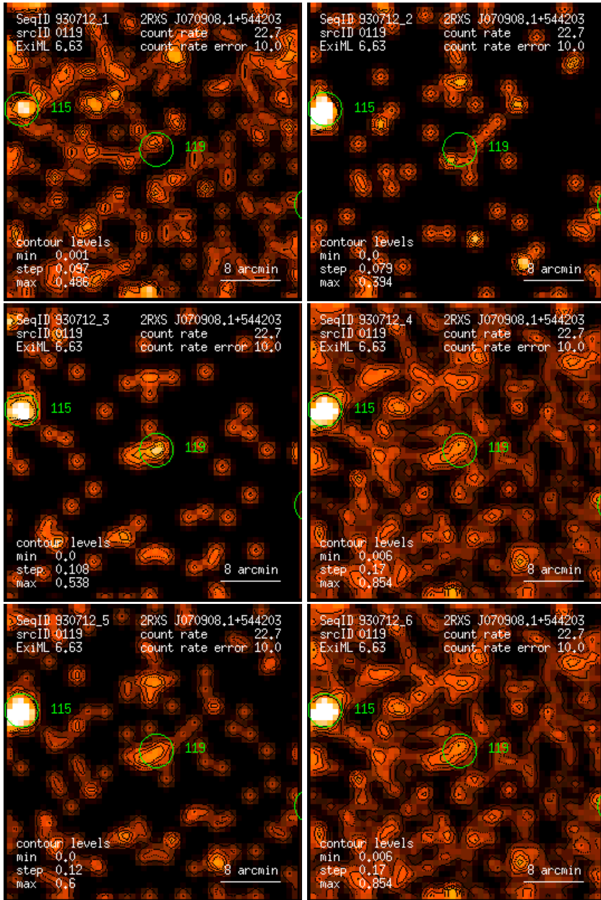
Figure 119: RASS 930712: detection 0119: band rate images, Gaussian filter: (1) PSPC channels 11 – 41, (2) 52 – 90, (3) 91 – 201, (4) 11 – 235, (5) 52 – 201, (6) 11 – 201. Broad band rates in counts/ks. Band rate contour levels in counts/ks/arcmin 2 .
