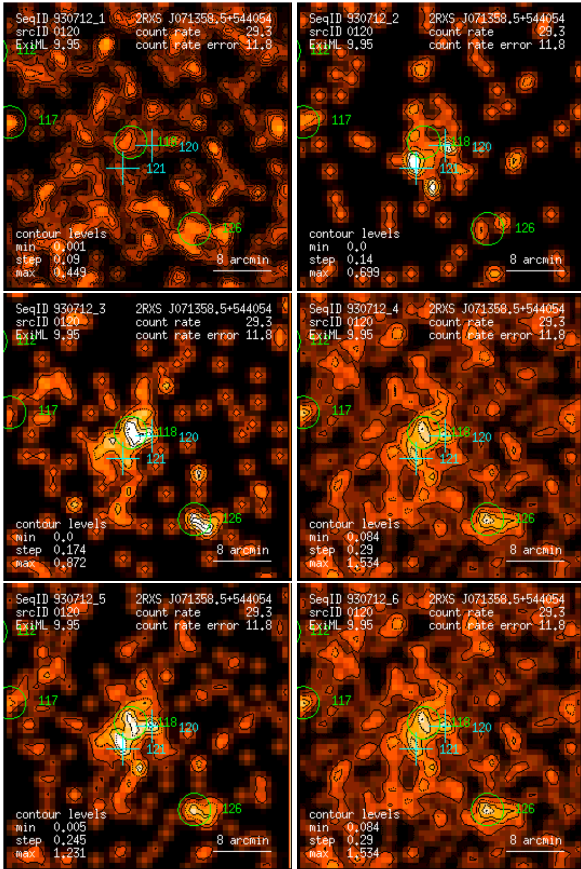
Figure 120: RASS 930712: detection 0120: band rate images, Gaussian filter: (1) PSPC channels 11 – 41, (2) 52 – 90, (3) 91 – 201, (4) 11 – 235, (5) 52 – 201, (6) 11 – 201. Broad band rates in counts/ks. Band rate contour levels in counts/ks/arcmin 2 .
