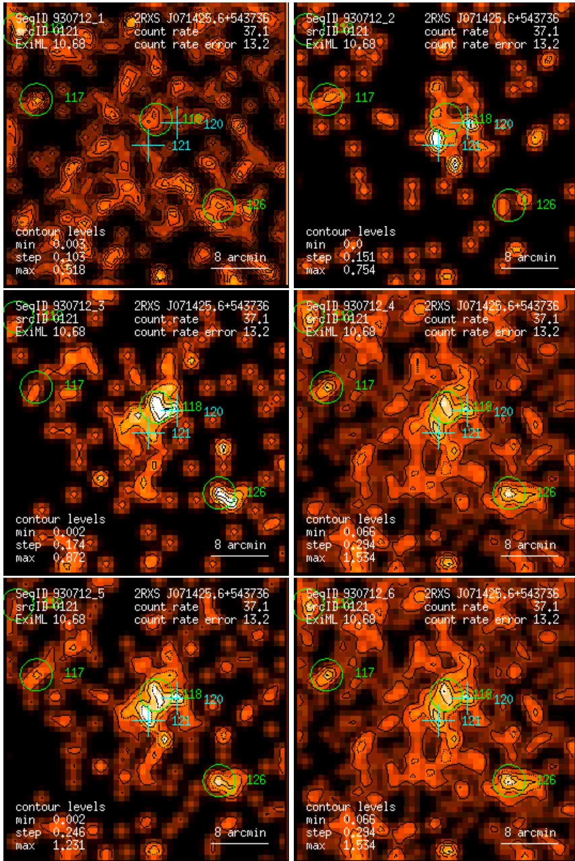
Figure 121: RASS 930712: detection 0121: band rate images, Gaussian filter: (1) PSPC channels 11 – 41, (2) 52 – 90, (3) 91 – 201, (4) 11 – 235, (5) 52 – 201, (6) 11 – 201. Broad band rates in counts/ks. Band rate contour levels in counts/ks/arcmin 2 .
