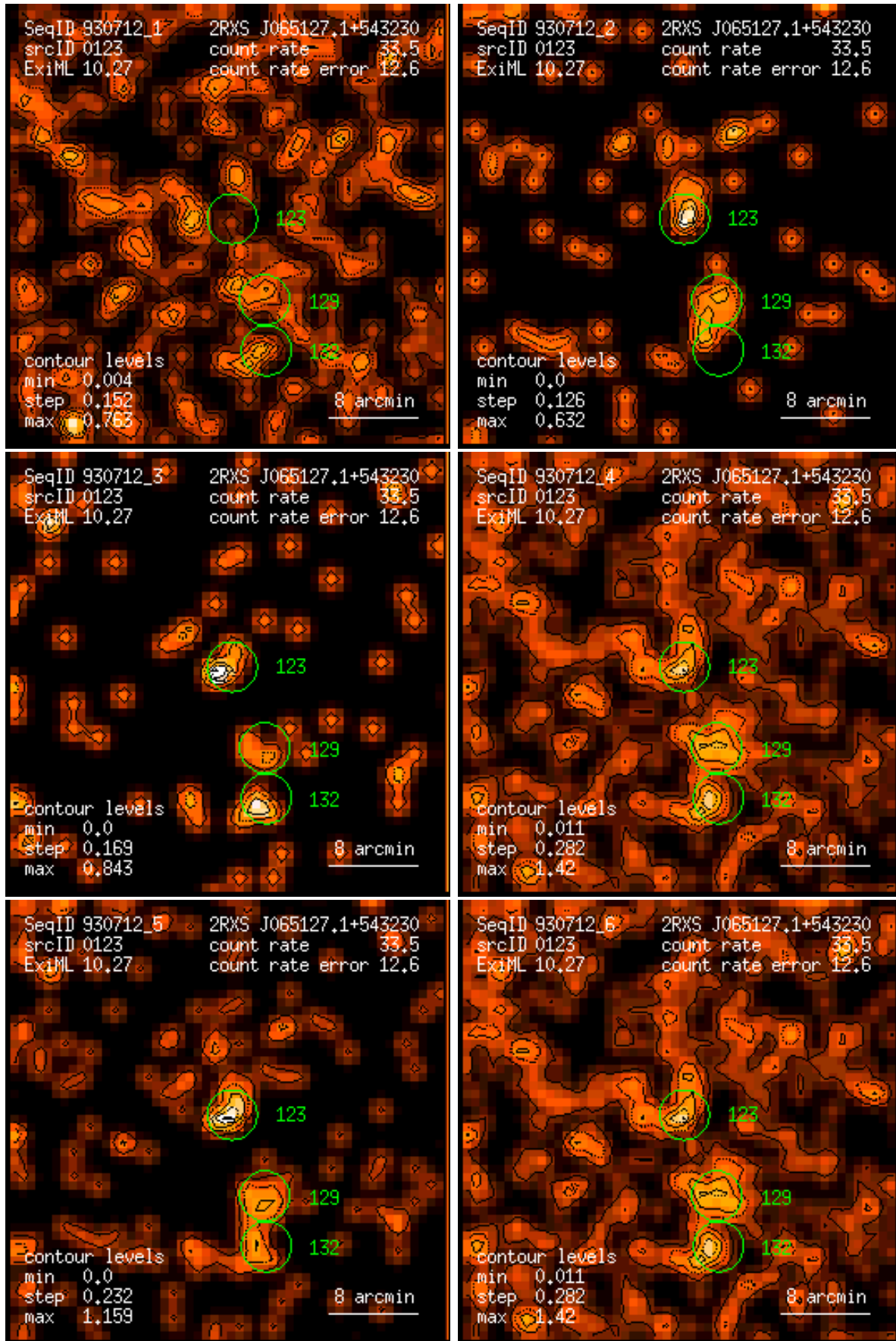
Figure 123: RASS 930712: detection 0123: band rate images, Gaussian filter: (1) PSPC channels 11 – 41, (2) 52 – 90, (3) 91 – 201, (4) 11 – 235, (5) 52 – 201, (6) 11 – 201. Broad band rates in counts/ks. Band rate contour levels in counts/ks/arcmin 2 .
