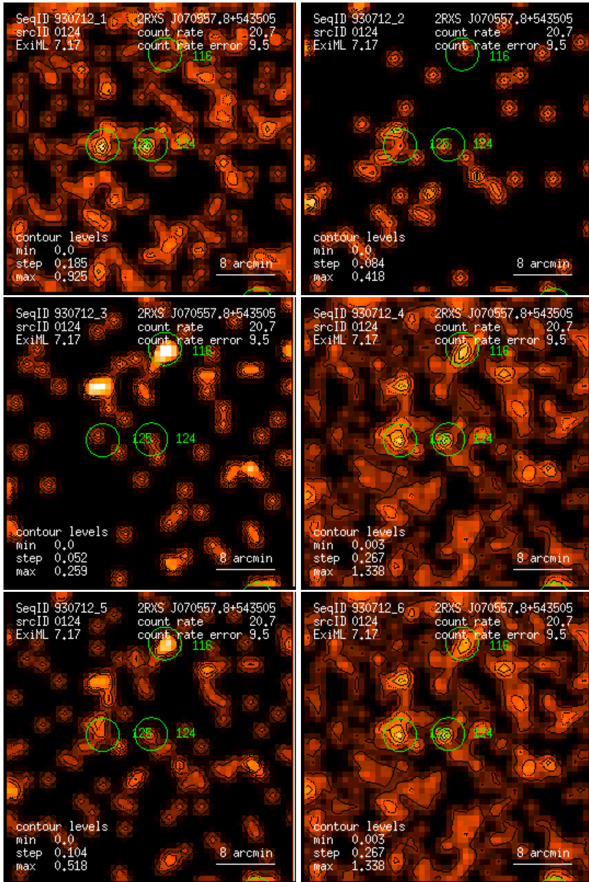
Figure 124: RASS 930712: detection 0124: band rate images, Gaussian filter: (1) PSPC channels 11 – 41, (2) 52 – 90, (3) 91 – 201, (4) 11 – 235, (5) 52 – 201, (6) 11 – 201. Broad band rates in counts/ks. Band rate contour levels in counts/ks/arcmin 2 .
