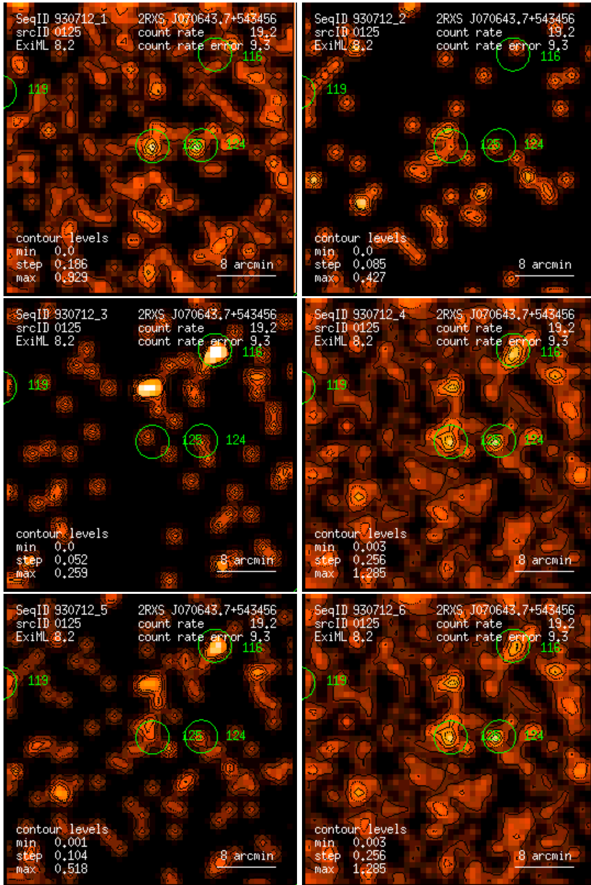
Figure 125: RASS 930712: detection 0125: band rate images, Gaussian filter: (1) PSPC channels 11 – 41, (2) 52 – 90, (3) 91 – 201, (4) 11 – 235, (5) 52 – 201, (6) 11 – 201. Broad band rates in counts/ks. Band rate contour levels in counts/ks/arcmin 2 .
