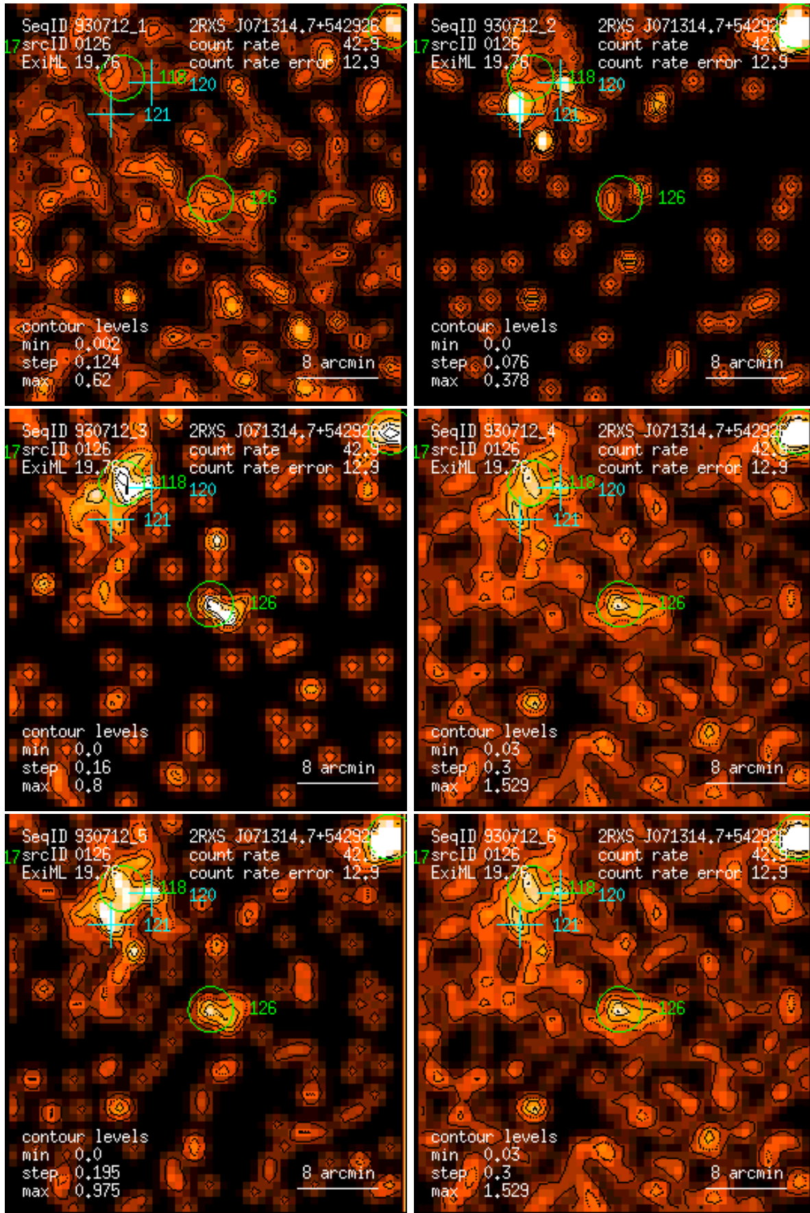
Figure 126: RASS 930712: detection 0126: band rate images, Gaussian filter: (1) PSPC channels 11 – 41, (2) 52 – 90, (3) 91 – 201, (4) 11 – 235, (5) 52 – 201, (6) 11 – 201. Broad band rates in counts/ks. Band rate contour levels in counts/ks/arcmin 2 .
