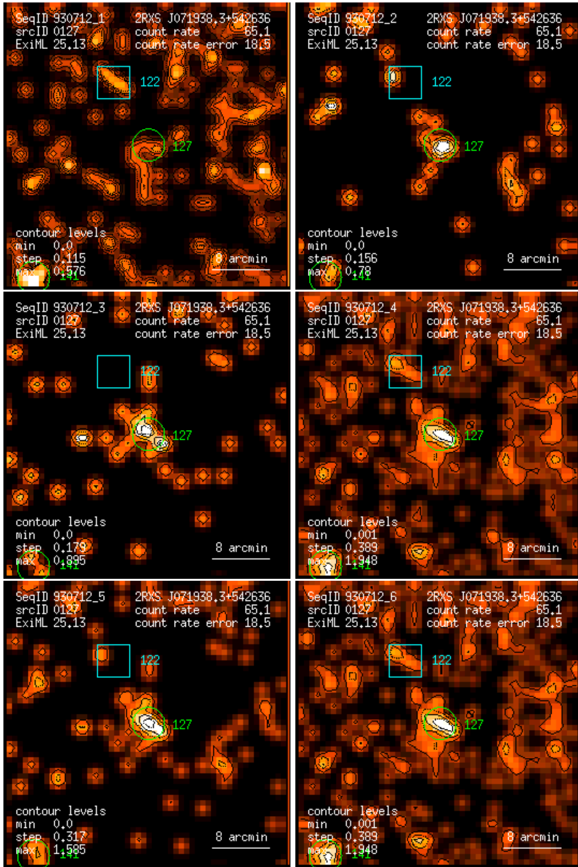
Figure 127: RASS 930712: detection 0127: band rate images, Gaussian filter: (1) PSPC channels 11 – 41, (2) 52 – 90, (3) 91 – 201, (4) 11 – 235, (5) 52 – 201, (6) 11 – 201. Broad band rates in counts/ks. Band rate contour levels in counts/ks/arcmin 2 .
